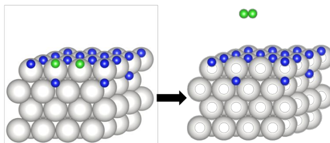
Figure 4. Depiction of possible desorption mechanism where two surface hydrogen (green balls) desorb from two fcc sites with a subsurface hydrogen atom in an oct site ( \theta = 1.0 , \theta_{\text{subsurface}} = 0.25 ). White = Cobalt, Blue = Hydrogen, Green = Hydrogen
