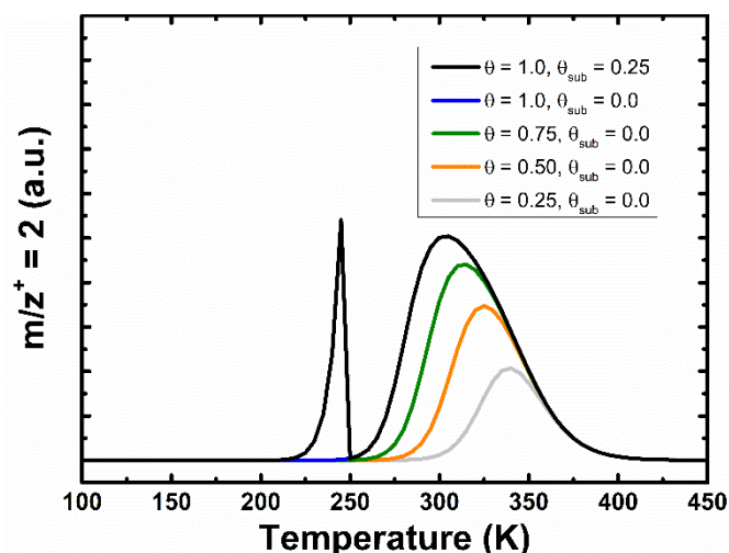
Figure 5. Simulated TPD spectra for hydrogen on Co(0001). Note: The black and blue features overlap above 250 K.
