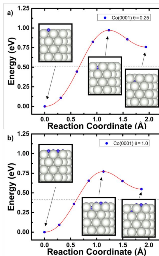
Figure 1. CI-NEB of diffusion of a single hydrogen from a surface fcc site to a subsurface octahedral site on a) clean ( \theta = 0.25 ) and b) hydrogen covered surface ( \theta = 1.0 ). The insets show the initial, saddle and final states. White spheres are cobalt, blue are hydrogen and the dashed line represents the reference energy level of a clean surface and H_2 in the gas phase.
