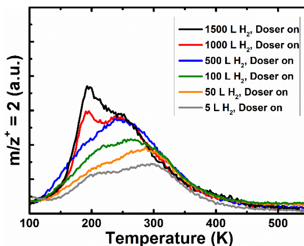
Figure 3. TPD after various exposures of excited hydrogen with the sample held at 100 K.
