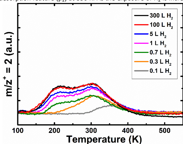
Figure 2. TPD after various exposures of hydrogen with the sample held at 100 K
