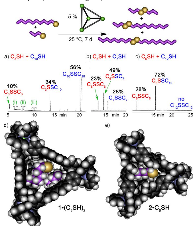
Figure 3. Size-selective Reactivity. Expansions of the GC traces obtained after reaction between different thiols (25 °C, 7 days, CD 3 CN, 5% 1 ). a) C 3 -SH and C 10 -SH; b) C 6 -SH and C 7 -SH; c) C 6 -SH and C 12 -SH. Minimized structures of d) 1•(C 8 -SH) 2 e) and 2•C 6 -SH (SPARTAN). (i): dodecane; (ii) unreacted C 10 -SH; (iii) impurity in the GC column.
