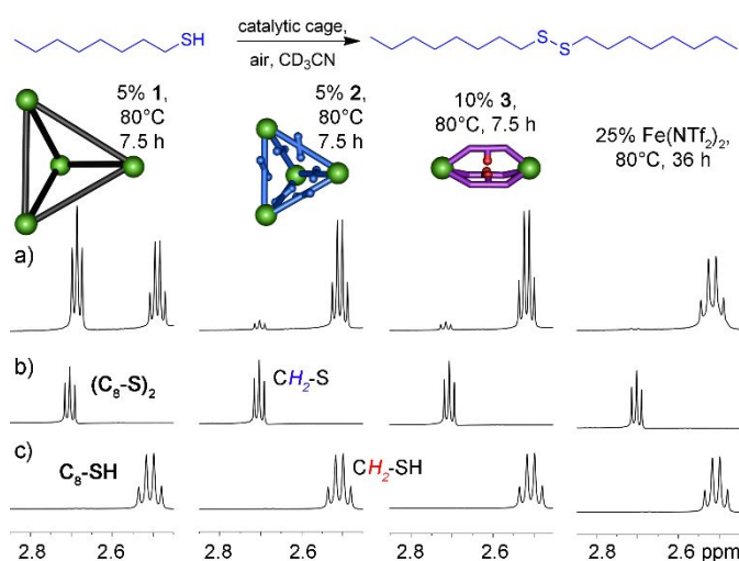
Figure 2. 1 H NMR analysis of the reaction catalyzed by various Fe-containing species. Expansion of the CH 2 -S region of the 1 H NMR spectra of a) reaction mixture after reaction for the indicated time; b) purified disulfide product (C 8 -S) 2 ; c) purified thiol starting material C 8 -SH. CD 3 CN, 400 MHz, spectra acquired at 298 K.
