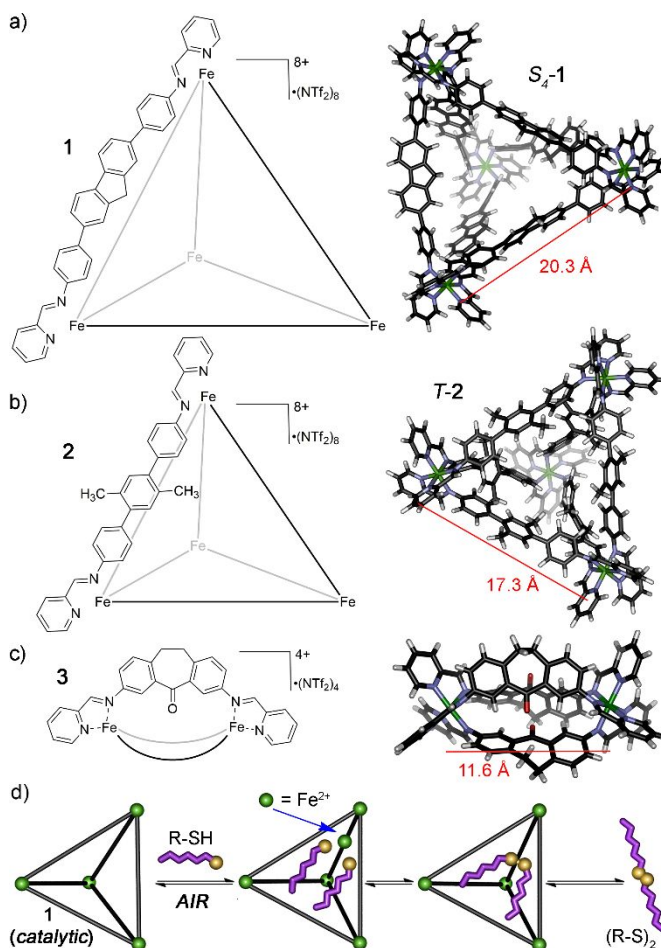
Figure 1. Self-assembled cage complexes tested. a) large Fe 4 L 6 host 1 ; b) medium-sized Fe 4 L 6 tetrahedron 2 ; c) Fe 4 L 6 helicate 3 . d) illustration of the oxidation process.
