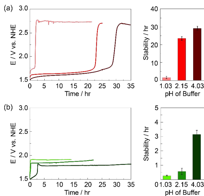
Figure 3. Stability of \text{CoFePbO}_x films performing OER at 1 \text{ mA/cm}^2 in solutions containing (a) 1 \text{ M KNO}_3 + 0.1 \text{ M KP}_i and (b) 1 \text{ M KNO}_3 + 0.1 \text{ M KS}_i at different pH: 1.03 (light red and light green), \text{pH} 2.15 (red and green), and \text{pH} 4.03 (dark red and dark green). Representative chronopotentiometry curves (left), and bar graphs indicating average film stabilities (right) at each pH are shown.
