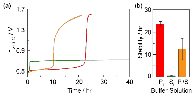
Figure 2. Stability of \text{CoFePbO}_x films performing OER at 1 \text{ mA/cm}^2 in buffer solutions (pH 2.15) of 1 \text{ M KNO}_3 + 0.1 \text{ M KP}_i (red, \text{P}_i ), 1 \text{ M KNO}_3 + 0.1 \text{ M KS}_i (green, \text{S}_i ), or 0.8 \text{ M KNO}_3 + 0.1 \text{ M KP}_i + 0.1 \text{ M KS}_i (orange, \text{P}_i/\text{S}_i ): (a) chronopotentiometry curves, and (b) bar graphs indicating average stability (time required to reach the plateau current). \eta_{\text{pH}2.15} = E_{\text{appl}} - E_{\text{therm}} where E_{\text{therm}} is the thermodynamic potential for water splitting at \text{pH} = 2.15 and E_{\text{appl}} = applied potential.
