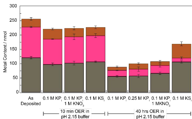
Figure 4. Total metal content, Pb (grey), Fe (brown), and Co (magenta) of 1 cm 2 CoFePbO x films after operation in specified buffers at pH 2.15 for 0 min, 10 min, or 40 h at 1 mA/cm 2 for OER.
