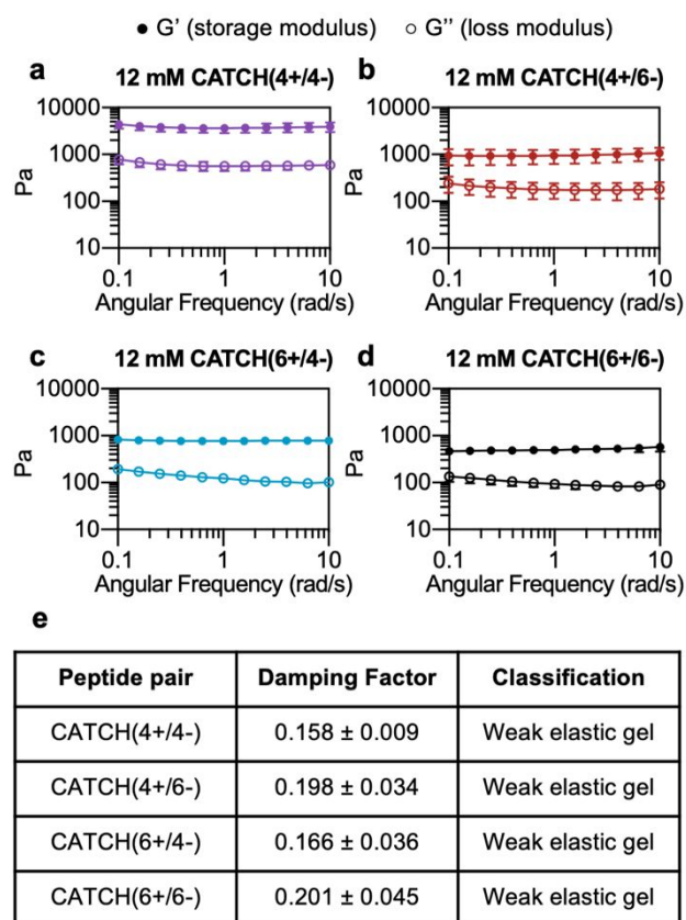
Figure 2. Oscillating rheology of CATCH(+/-) peptide hydrogels. (a-d) G' and G'' of 12 mM CATCH(4+/4-), CATCH(4+/6-), CATCH(6+/4-), and CATCH (6+/6-) hydrogels at different angular frequencies. (e) Average damping factor of 12 mM CATCH(+/-) hydrogels, calculated as the average of the G''/G' ratio at each angular frequency. Data are presented as the mean \pm standard deviation ( n = 3 ).
