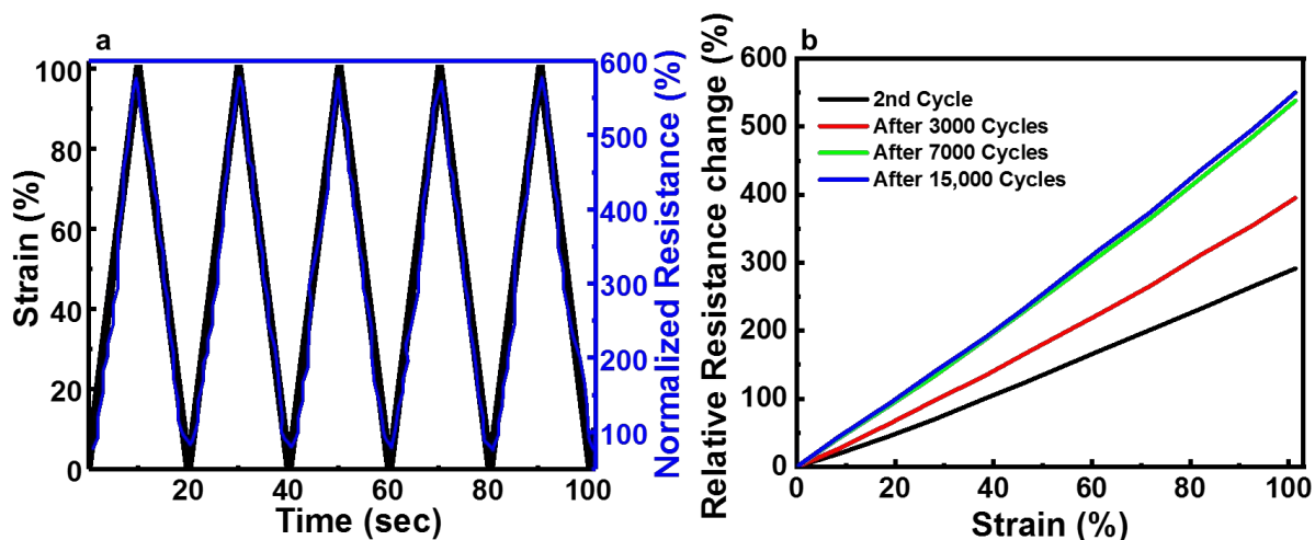
Fig. 5 (a) Normalized resistance change of the sensor after 15,000 cycles in response to applied strain of 100%. (b) Relative resistance change with strain after particular cycles during cycling stability testing of the sensor.
