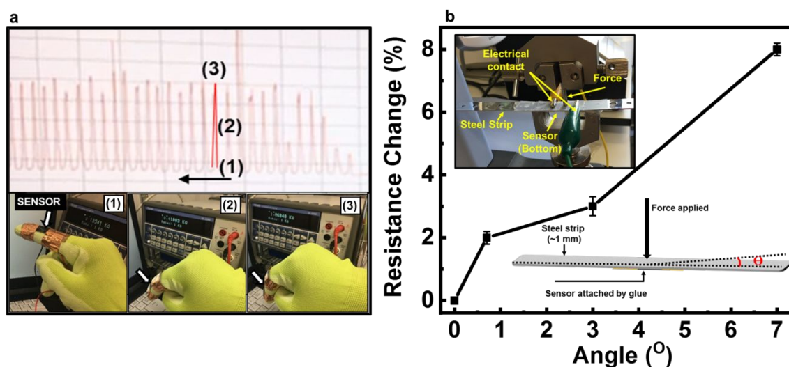
Fig. 6 (a) Real-time response of the sensor in detecting human finger motion. (b) Resistance change during strain detection (change in angle, degree) of a steel strip connected with fabricated sensor.
