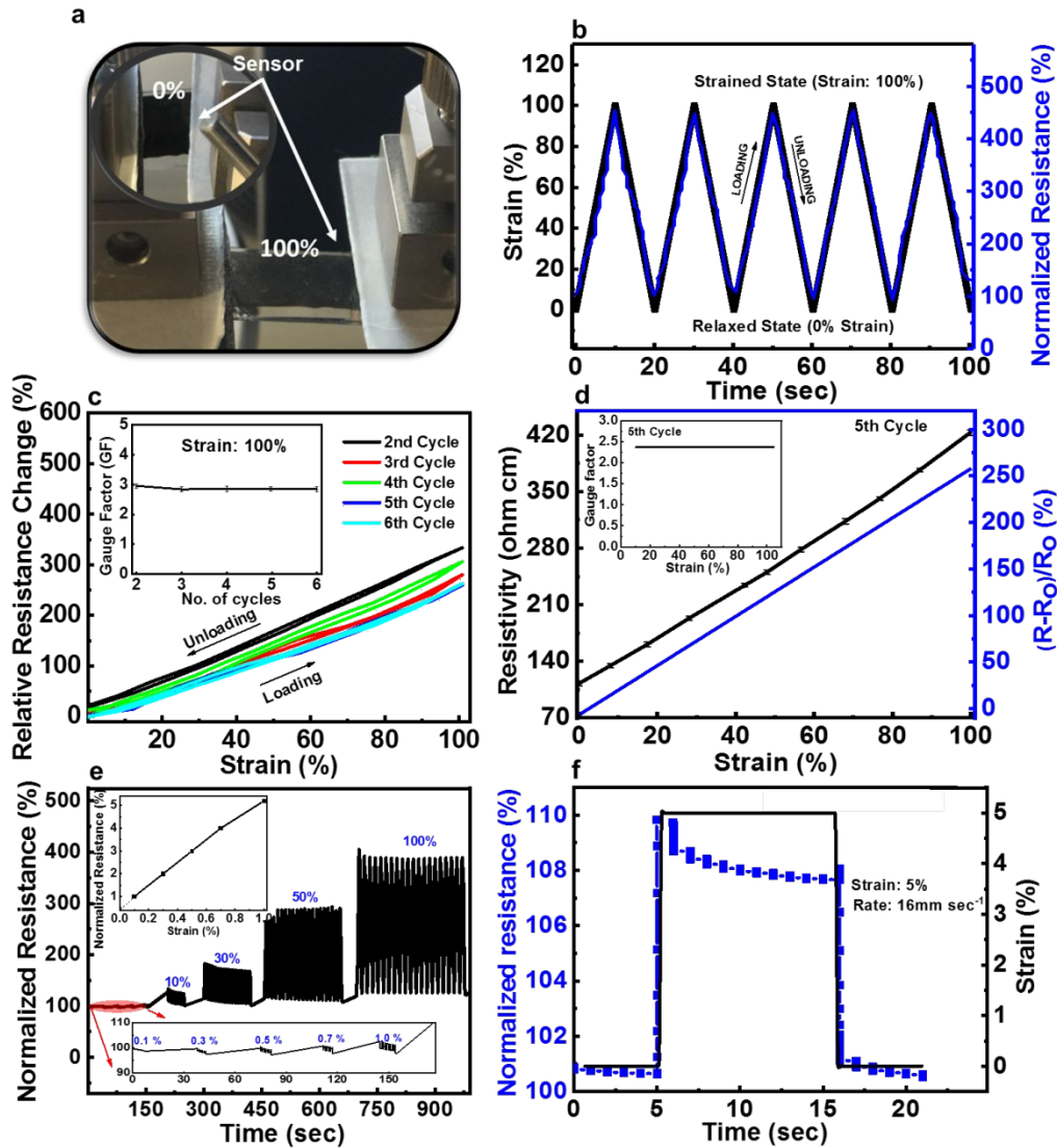
Fig. 3 (a) Image of sensor at 0% and 100% strain. (b) Relative resistance change and strain variation with time during initial cycling of sensor. (c) Resistivity change with strain for six consecutive initial cycles. (d) Resistivity and relative resistance change of sensor with strain (5 th cycle) showing a highly linear response. (e) Normalized resistance change with increasing strain. (f) Response time of the sensor during quasi-transient loading (5% strain at 16 mm sec -1 ).
