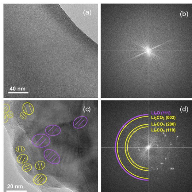
Figure 5. Cryo-EM image (a) and FFT pattern (b) of polyVC-LiI gel electrolyte. Cryo-EM image (c) and FFT pattern (d) of the SEI layer on Li metal after Li//Li symmetric cycling for 10 cycles at 1 \text{ mA cm}^{-2} , 1 \text{ mAh cm}^{-2} . Direction of the lattice planes in each crystal grain are emphasized by the straight lines.
