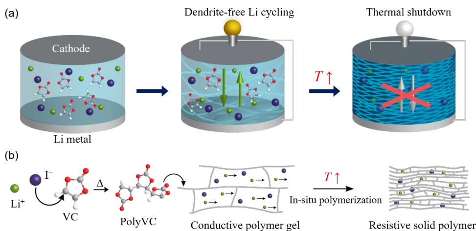
Figure 1. (a) Li metal battery enabling dendrite-free Li cycling at room temperature and thermal shutdown when temperatures increase. (b) Chemical reactions and physical state of the polyVC-LiI gel inside the battery represented in (a). Heating of the electrolyte within a controlled time triggers partial polymerizations of VC with I - anion to form the polymer gel network. Prolonged time of heating leads to full polymerization of VC and results in the resistive solid phase.
