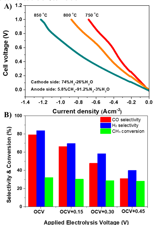
Figure 4 A) i - V curves of Ru infiltrated electrolyzer for POM assisted steam electrolysis measured at 750-850 °C, and B) CH 4 conversion, CO selectivity and H 2 selectivity in the anode of the electrolyzer operated in POM assisted mode at 850 °C. During the operation, the anode and the cathode are exposed to 5.8%CH 4 -91.2%N 2 -3%H 2 O and 74%H 2 -26%H 2 O atmosphere, respectively.
