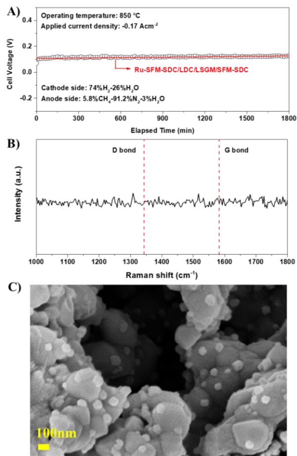
Figure 6 A) Durability of Ru infiltrated single cell for methane assisted steam electrolysis process at 850 °C and an electrolysis current density of -0.17\text{Acm}^{-2} , B) Raman spectrum, and C) SEM image of the post-test Ru infiltrated SFM-SDC electrode.
