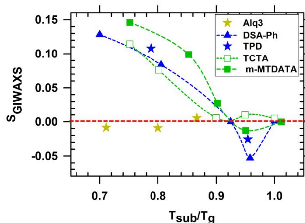
Figure 4: The S_{GIWAXS} order parameter as a function of substrate temperature plotted for vapor-deposited glasses made from rod-shaped TPD and DSA-Ph, disk-shaped m-MTDATA and TCTA and spheroidal shaped Alq3. The GIWAXS order parameter reported here is a measure of anisotropic structure of the bulk glass. Also note that the Alq3 order parameter characterizes the scattering at \sim 1.6 \text{ \AA}^{-1} , and not the scattering feature at 0.8 \text{ \AA}^{-1} . The average error in the order parameter, determined from repeating a subset of experiments (both sample preparation and GIWAXS measurement) is \sim 0.007 .
