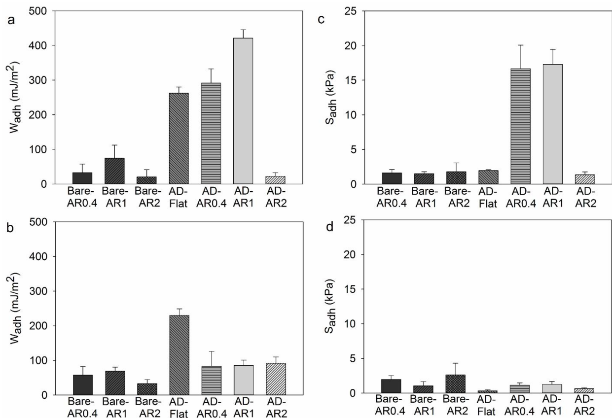
Figure 4. W_{adh} (a, b) and S_{adh} (c, d) for adhesive tested at pH 3 (a, c) and 9 (b, d) ( n = 3 ). Refer to Tables S1 and S2 for statistical analysis.
