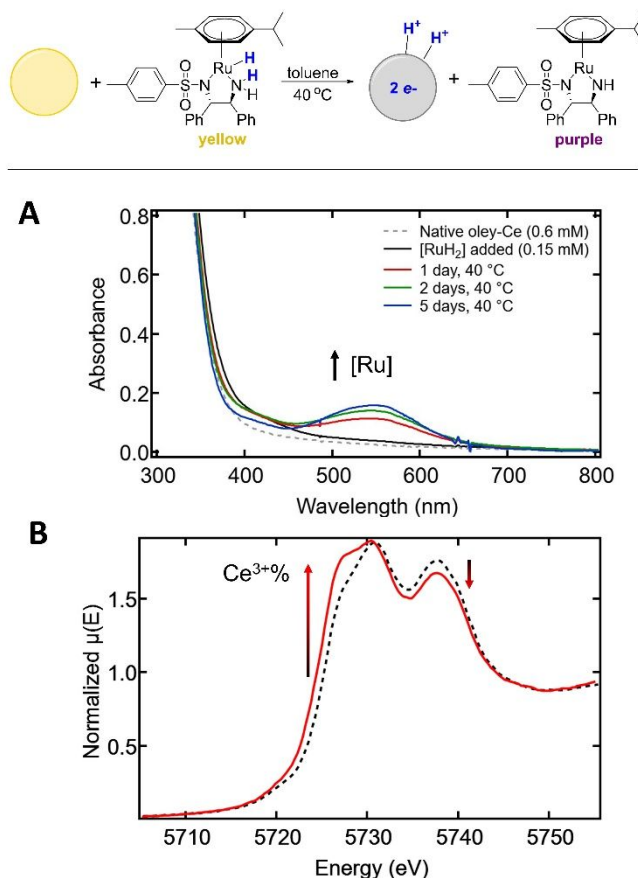
Figure 1. A) UV-visible spectra following the reaction of [RuH 2 ] with oley-Ce NPs (shown at the top) in toluene at 40 °C over several days. B) Complimentary XAS data of the hydride reaction over 24 hours (red) at the Ce-L 3 edge shows an increase of Ce 3+ % in comparison to the native nanoparticles (black).
