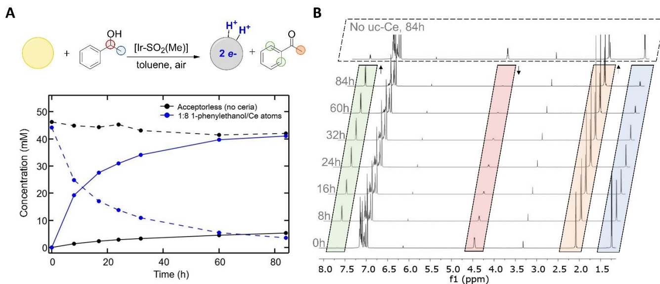
Figure 4. Aerobic oxidation of 1-phenylethanol. A) Plot of concentration of alcohol (dashed lines) and ketone product (solid lines) as a function of time for the full catalytic system (blue) and for the parallel control without any ceria (black). B) ^1\text{H} NMR spectra of an aerobic oxidation of 1-phenylethanol with [\text{Ir-SO}_2(\text{Me})] and uc-Ce in toluene at 80 °C. Reactions were run in a J-Young NMR tube and opened to air to replenish \text{O}_2 each time they were cooled to collect a spectrum. Spectra from 0 to 84 h of reaction time are stacked, and the top spectrum is from an independent reaction without any added uc-Ce under parallel conditions. The solid colors beneath the peaks refer to the resonances highlighted in the chemical equation.
