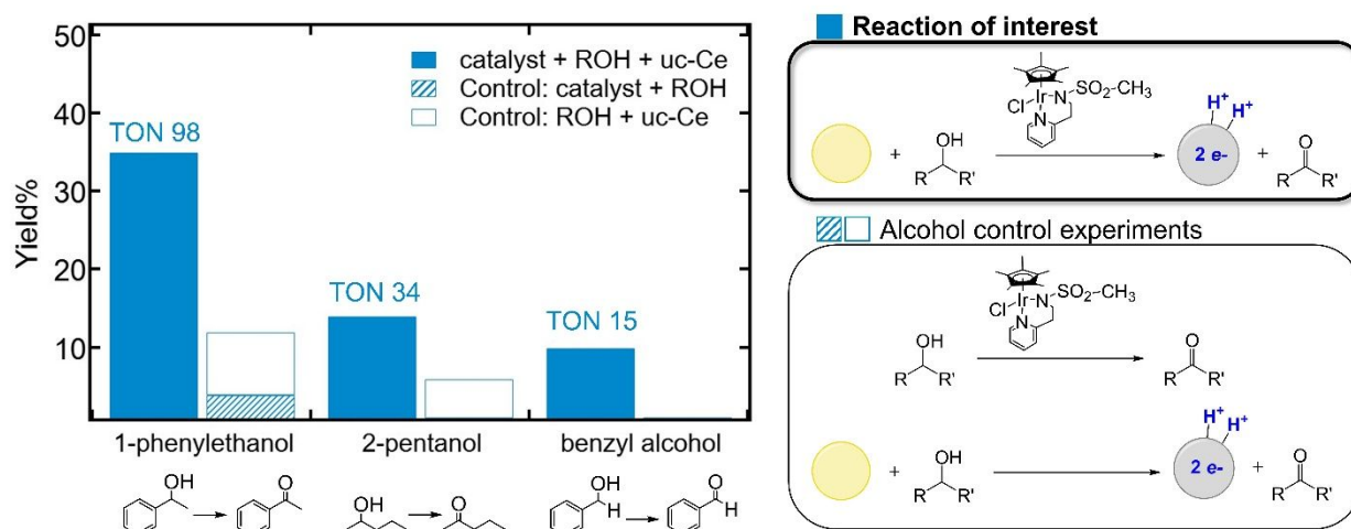
Figure 3. Yields of ketone or aldehyde products from the catalytic oxidation and control reactions of 1-phenylethanol, 2-pentanol and benzyl alcohol. The reaction of interest (solid blue bars) utilizes the [Ir-SO 2 (Me)] catalyst and uc-Ce as an acceptor under anaerobic conditions in the stoichiometry of [Ir-SO 2 (Me)] : ROH : Ce atoms = 0.55 : 100 : 800. The corresponding TON for the complete catalytic reaction is given above the solid blue bar. The striped bars correspond to the control reaction of [Ir-SO 2 (Me)] and alcohol (<9 TONs for all cases), while the blank bars correspond to the control reaction of uc-Ce and alcohol. The results of the two control experiments (striped and blank bars) are stacked to show that the sum of their yields was less than those of the complete uc-Ce/[Ir-SO 2 (Me)] catalytic system.
