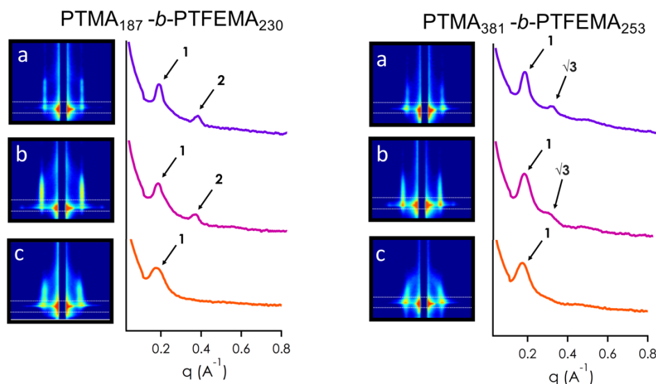
Figure 4 2D-GISAXS data for PTMA 187 - b -PTFEMA 230 and PTMA 381 - b -PTFEMA 253 thin films annealed for 6 hrs in chloroform vapor. Data represented showed thin films where (a) RTP-1 was used as an underlayer, (b) RTP-2 was used and (c) no underlayer was used.
