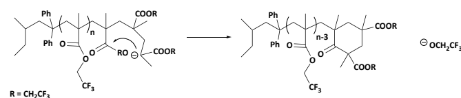
Scheme 2 Plausible termination via backbiting of PTFEMA.
