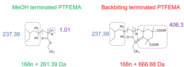
Scheme 3 Species and respective molar masses of PTFEMA chains properly terminated by degassed MeOH and those terminated due to backbiting.
