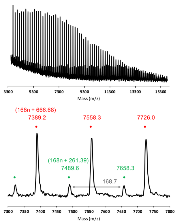
Figure 1 MALDI-TOF-MS spectrum of PTFEMA synthesized with a \text{Li}^+ counteranion with excess \text{LiCl} .
