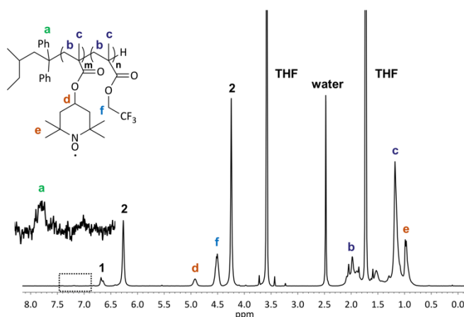
Figure 2 1 H NMR spectrum of PTMA 381 - b -PTFEMA 253 measured in THF d-8 after reduction with pentafluorophenylhydrazine (PFPhHz). Signals attributable to the N-OH group (converted from NO•) are assigned as 1 . The PFPhHz signals are marked as 2 .
