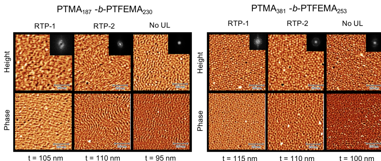
Figure 3 AFM images of PTMA 187 - b -PTFEMA 230 and PTMA 381 - b -PTFEMA 253 thin films annealed for 6 hr in chloroform vapor. The height and phase images are shown for films in which underlayers (RTP-1 and RTP-2) were used, and those which were not. Film thicknesses ( t ) are noted at the bottom of each figure.
