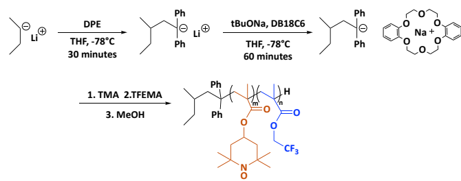
Scheme 1 Synthesis of PTMA- b -PTFEMA block copolymers by anionic polymerization using a Na + /DB18C6 counteraction and sequential monomer addition.
