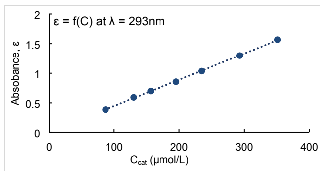
Figure 3. Absorbance of 1-Pd-NH 2 PEG at \lambda_{\text{max}} = 293 nm as a function of concentration.
