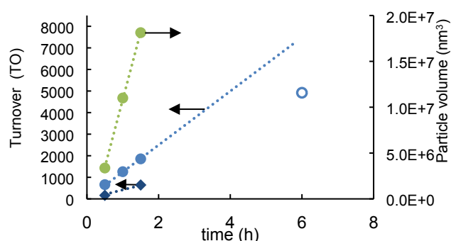
Figure 4. Study of the catalyst activity in blue (● 0.8 g/mL Rhodafac ® , ○ 1.6 g/mL Rhodafac ® and ◆ 0.75 g/mL SDS) and particle size as a function of time in green (● Rhodafac ® ).
