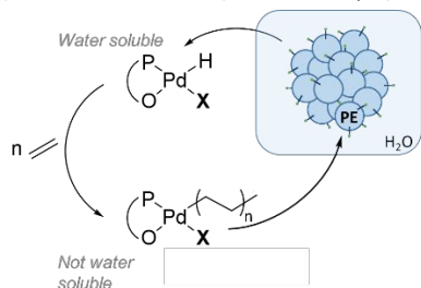
Figure 6. Schematic of proposed mechanism showing shuttling of catalyst between the water phase and the polymer particle.
