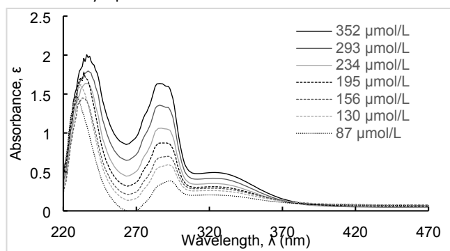
Figure 2. Ultraviolet-visible (UV) absorbance calibration of 1-Pd-NH 2 PEG in water/Rhodafac ® at different concentrations.
