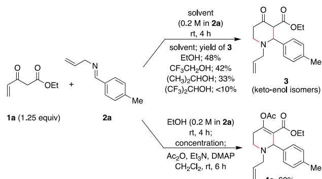
Scheme 2 Protic Solvent-Mediated aza-Annulation Reaction and Facile Derivatization to Enol Acetate.
