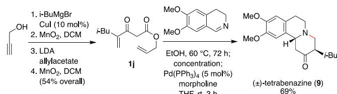
Scheme 4 Concise Synthesis of ( \pm )-Tetrabenazine from Propargyl Alcohol.
