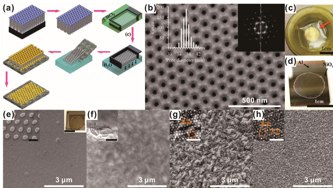
Figure 2 Fabrication of a nanodot array based on the template-assisted method. (a) Illustration of the fabrication process of an AAO pattern template using ultrathin alumina membranes (UTAM). (b) SEM image of the fabricated template. (c) Digital image of the fabricated template floating on water. (d) Transfer of the fabricated template. (e) SEM image of fabricated nickel nanodot arrays using a template. (f) Plain and oblique view an SEM image of transferred nanodot arrays. (g, h) Fabrication of gold nanodot arrays using a template-assisted method on an FTO substrate (g) and an ITO substrate (h). Scale bars in inset images of (e)–(h) are 500 nm. Reprinted with permission from ref. 60. Copyright © 2016 American Chemical Society.
