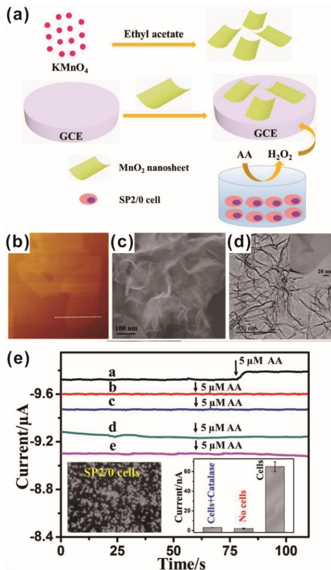
Figure 5 Non-destructive, live-cell monitoring technique by \text{H}_2\text{O}_2 monitoring using \text{MnO}_2 nanosheets on a glass carbon electrode (GCE). (a) Schematic illustration of \text{H}_2\text{O}_2 detection from SP2/0 cells. (b-d) Characterization of \text{MnO}_2 nanosheets. (e) Amperometric i - t curves of the response of GCE with \text{MnO}_2 nanosheets (curve a) and without \text{MnO}_2 nanosheets (curve d) for the reduction of \text{H}_2\text{O}_2 released from SP2/0 cells. Amperometric i - t curves of the response of GCE with \text{MnO}_2 nanosheets (curve b) and without \text{MnO}_2 nanosheets (curve e) in the absence of SP2/0 cells. Amperometric i - t curves of the response of GCE with \text{MnO}_2 nanosheets (curve c) in the presence of SP2/0 cells and catalase. Reprinted with permission from ref. 91. © 2017 Elsevier B.V. All rights reserved.
