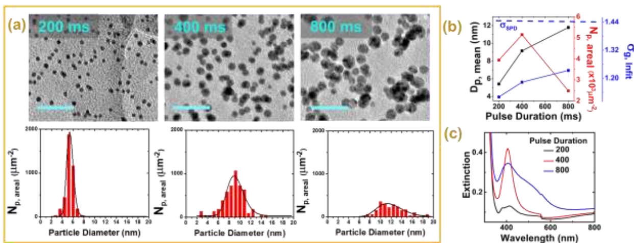
Figure 6. (a) TEM images (scale bar: 50 nm) and corresponding PSDs of Ag sMNPs-9kPVA films fabricated for different pulse duration for laser energy flux of 20 \text{ W cm}^{-2} , (b) Effect of pulse duration on mean particle diameter, geometric standard deviation ( \sigma_g ), and areal mass density in 9kPVA films, (c) Extinction spectra of Ag sMNPs-PVA films fabricated by LPSW for different number of pulses. Substrate used in 1 mm glass slide.
