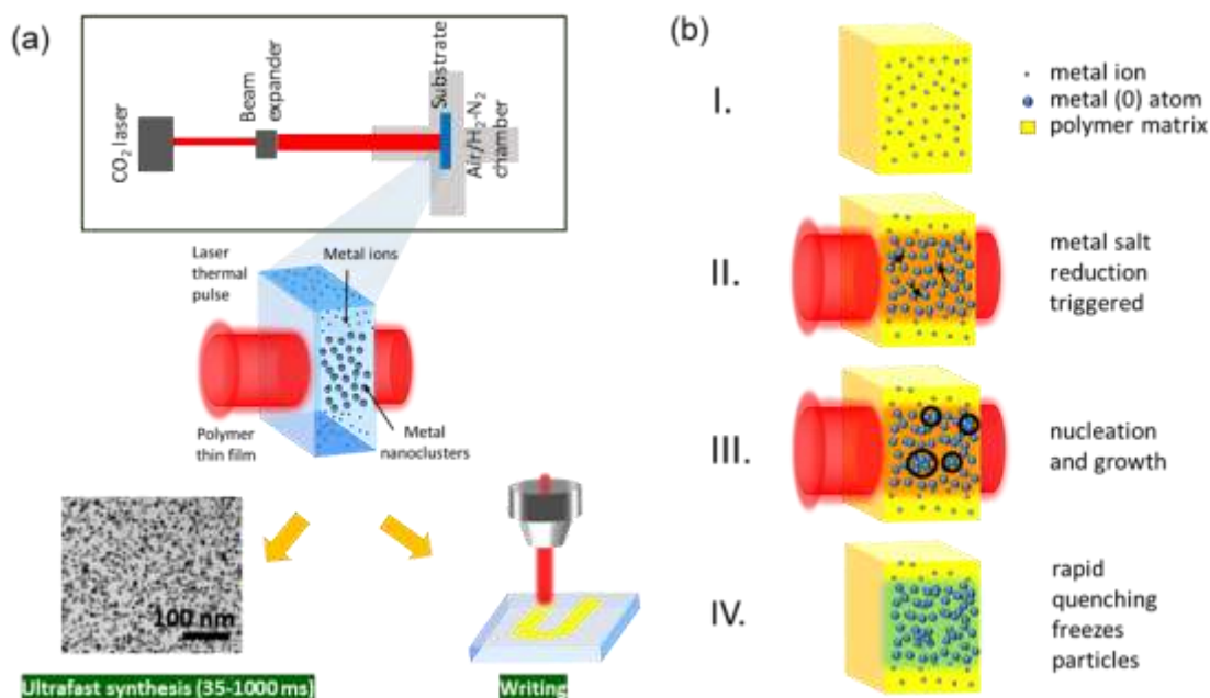
Figure 1. (a) Schematic showing laser photothermal synthesis and writing (LPSW) to form small metal nanoclusters directly in polymer thin film. (b) Basic mechanism of nanocluster formation by LPSW.
