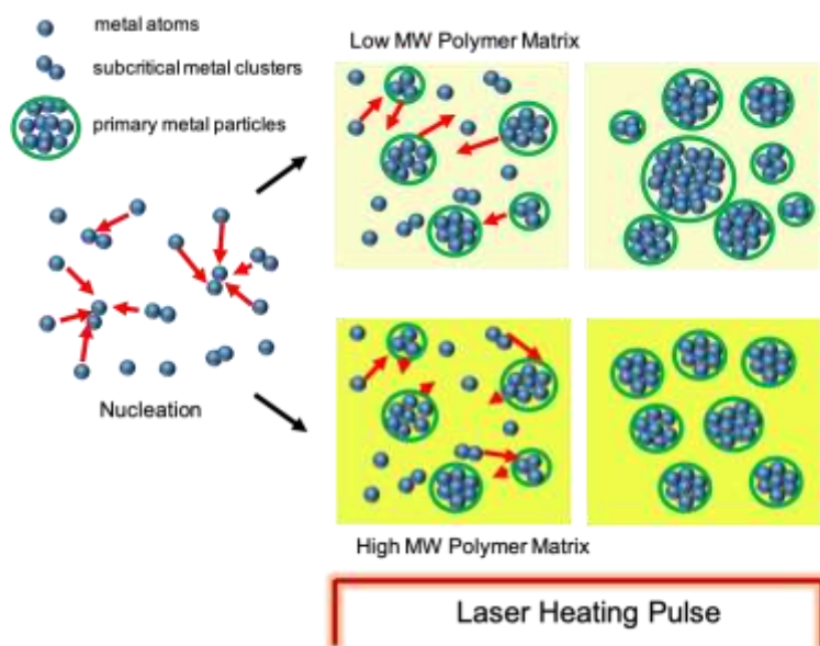
Figure 7. Primary growth mechanisms in LPSW of metal particles in polymer matrices with different molecular masses, resulting in two different kinds of size distributions.
