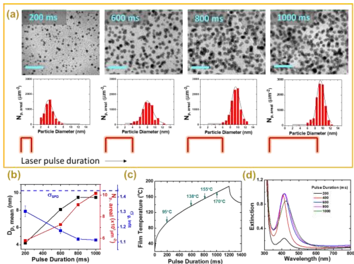
Figure 3. (a) TEM images (scale bars: 50 nm) and corresponding PSDs of Ag sMNPs-PVA films fabricated for different laser pulse duration for a fixed laser energy flux of 20 \text{ W cm}^{-2} , (b) Effect of pulse duration on mean particle diameter, areal particle mass density, geometric standard deviation ( \sigma_g , \ln(\text{fit}) ) obtained from lognormally fit PSDs, (c) Simulated temperature profile of laser
