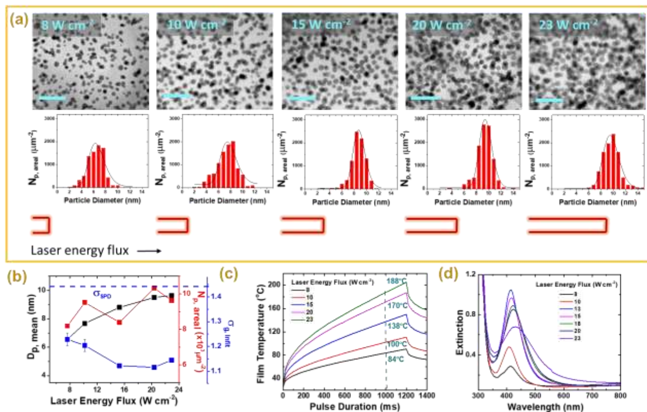
Figure 4. (a) TEM images (scale bar: 50 nm) and corresponding PSDs of Ag sMNPs-PVA films fabricated for different laser energy flux for a fixed pulse duration of 1000 ms, (b) Effect of laser energy flux on mean particle diameter and geometric standard deviation ( \sigma_{g, \ln fit} ) obtained from lognormally fit PSDs, (c) Simulated temperature profile of laser heating process with varying energy flux, (d) Extinction spectra of Ag sMNPs-PVA films fabricated by LPSW for different laser energy flux. Substrate used is 1 mm glass slide.
