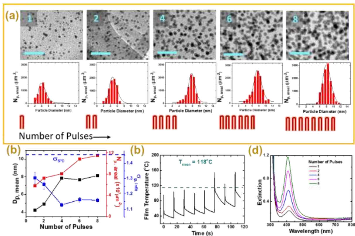
Figure 5. (a) TEM images (scale bar: 50 nm) and corresponding PSDs of Ag sMNPs-PVA films fabricated for different laser pulses ; 20 \text{ W cm}^{-2} , 1000 ms pulses, (b) Effect of number of input pulses on mean particle diameter and geometric standard deviation ( \sigma_g ) obtained from lognormally fit PSDs, (c) Simulated temperature profile of laser heating process with periodic heat load, (d) Extinction spectra of Ag sMNPs-PVA films fabricated by LPSW for different number of pulses. Substrate used is 1 mm glass slide.
