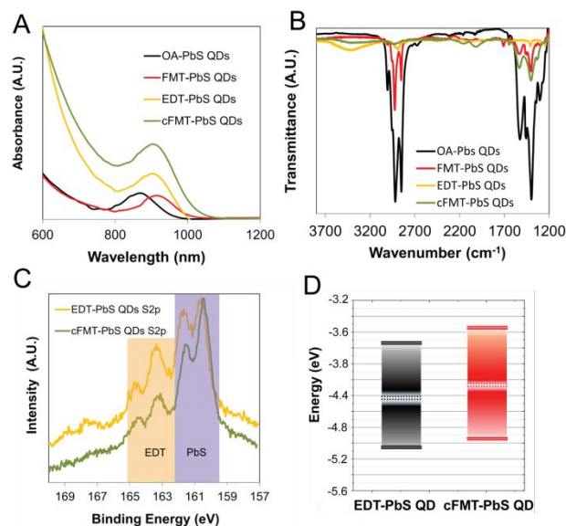
Figure 2: A) Absorbance spectra of QD films: OA-PbS (black), FMT-PbS (red), EDT-PbS films made by the conventional method (yellow), and cFMT-PbS films made by the conventional method (green). B) FTIR spectra QD films: OA-PbS (black, scaled to one third intensity for comparison), FMT-PbS (red), EDT-PbS films made by the conventional method (yellow), and cFMT-PbS films (green). C) XPS sulfur 2p spectra comparing the EDT-PbS film (yellow) and cFMT-PbS film (green) D) Band structure determined by UPS and absorbance results comparing the band alignments of an EDT-PbS film (black) and a cFMT-PbS film (red).
