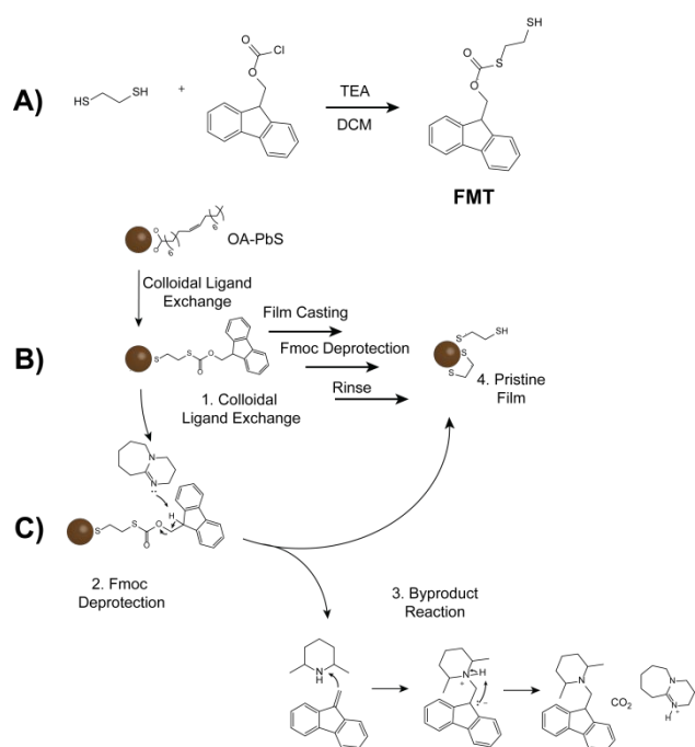
Figure 1: A) Synthesis of FMT. B) Schematic illustration showing PbS thin film formation. Pristine oleic acid (OA)-capped PbS is exchanged in solution with FMT. After the facile cleavage with a base, byproducts are removed leaving behind only EDT. C) Mechanism of Fmoc deprotection.
