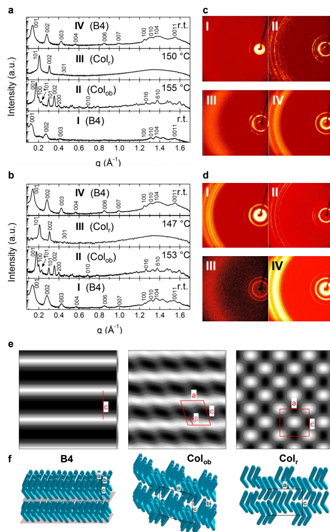
Fig. 3. X-ray diffraction analysis of slow heated and cooled (at 5 °C min -1 ) samples of: (a, c) p -( R )- 4 and (b, d) p -( S )- 4 ; (a, b) azimuthally integrated intensity (a.u.) vs. q ( \text{\AA}^{-1} ) of (c, d) the corresponding 2D diffraction patterns. Additional synchrotron small angle X-ray diffraction experiments were used to index the B4 (HLNC) and Col ob phases (see ESI, Section 8, Fig. S18 and Table S2). (e) 2-Dimensional electron density maps reconstructed from X-ray data by reverse Fourier transform of the B4 (HLNC), Col ob and Col r phases. Maps show ac plane. The change from black to white indicates increasing electron density. The modulation in-layer along the 'a' direction for the B4 phase is equal a single molecule and therefore not visible. The size of these maps is 15 × 15 nm 2 . The isodensity line is marked to visualize the cross section of the columns. (f) Corresponding molecular models for the B4, Col ob and Col r phase formed by p -( R )- 4 and p -( S )- 4 .
