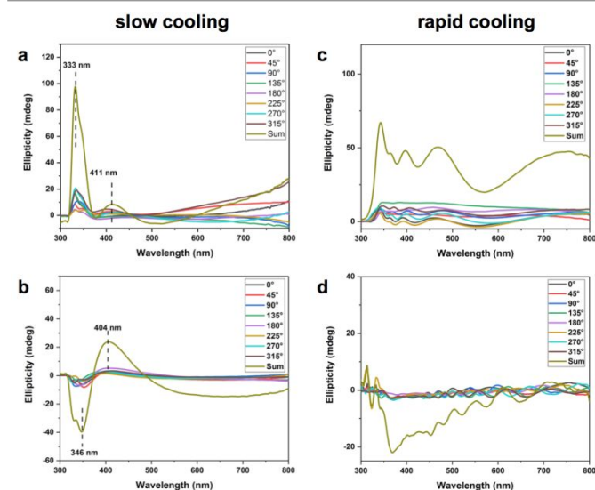
Fig. 2. Thin film CD spectra (film thickness: 10 μm) of: (a, c) p -( R )- 4 and (b, d) p -( S )- 4 on: (a, b) slow and (c, d) rapid cooling from the isotropic liquid phase to room temperature (r.t.). Sum and individual sample rotation spectra are shown.
