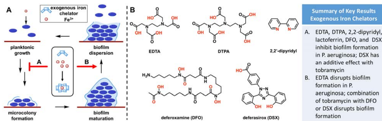
Figure 2. (A) Effect of exogenous iron chelators on biofilm formation. Some compounds inhibit formation of biofilms, while others induce biofilm dispersion. (B) Structures of relevant exogenous iron chelators. Chelating atoms are highlighted in red.
