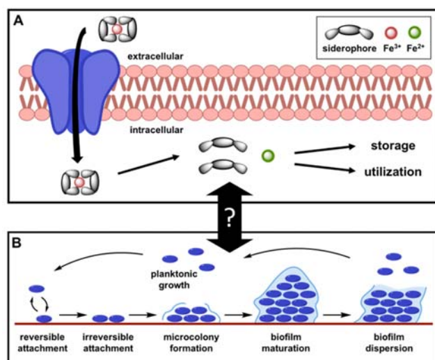
Figure 1. (A) Overview of iron acquisition by siderophores. (B) Steps in biofilm formation.
