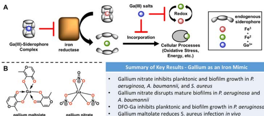
Figure 3. (A) Effect of gallium treatments on iron utilization. Gallium-siderophore complexes inhibit iron-reductase. Gallium salts inhibit other iron-dependent redox processes. (B) Structures of relevant gallium and iron complexes. Chelating atoms are highlighted in red.
