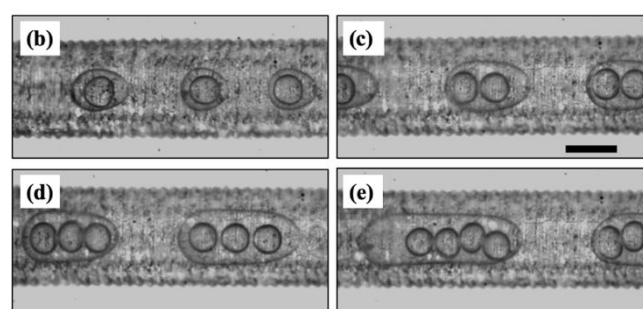
Fig. 5 (a) Variation in Q_i to produce double emulsions with various sizes of core drops, which are highlighted in red in the images of the double emulsion drops shown. Q_o is simultaneously varied to produce single-core double emulsions for each value of Q_i . For each Q_i , the average size of the core drop and outer drop are indicated in filled red and orange circles, respectively. Error bar represents standard deviation of the size for 20 replicates. Q_o is indicated using an unfilled blue diamond. For clarity, we have used a dashed yellow line to indicate each set of core size, outer size, and Q_o . Scale-bar represents 200 \mu\text{m} . (b-e) Monodisperse W/O/W double emulsions with different numbers of core drops of the inner phase. Q_i and Q_m are both kept constant at 1000 \mu\text{l/h} . Double emulsions with (b) one core where Q_o = 3500 \mu\text{l/h} , (b) two cores where Q_o = 2500 \mu\text{l/h} , (c) three cores where Q_o = 2000 \mu\text{l/h} , and (d) four cores where Q_o = 1600 \mu\text{l/h} . Scale-bar represents 500 \mu\text{m} .
