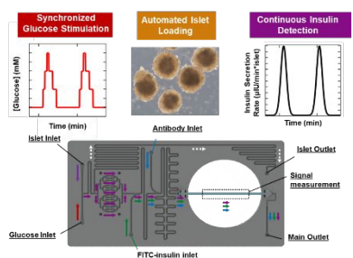
A device engineered from scalable materials for automated islet loading, synchronized stimulus delivery, and continuous on-chip insulin detection
