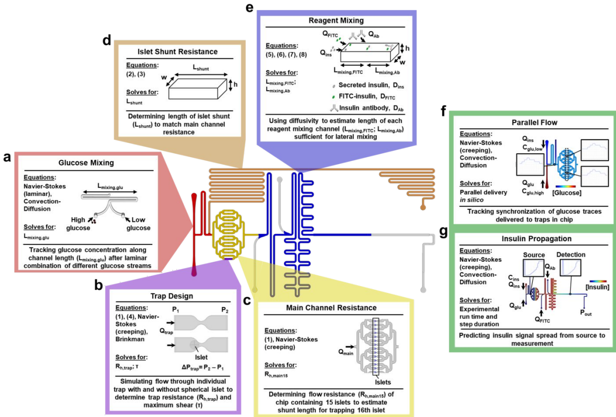
Figure 2 | Modeling for chip feature design. Graphical schematic outlining the model design for the ‘Islet on a Chip’ with specific regions highlighted. a. Glucose mixing channel. Three-dimensional flow and convection-diffusion modeled using CAD to ensure sufficient channel length ( L_{mixing,glu} ) for complete mixing of glucose input streams. b. Islet trap. Single traps were modeled with three-dimensional flow simulations to predict changes in pressure ( \Delta P ), flow rate ( Q_{trap} ), resistance, and shear ( \tau ) in the presence and absence of islets. Traps were designed to maximize inward flow, while retaining minimal shear. c. Main channels. Hydraulic resistance ( R_{main} ) through main chip channels was modeled with 15 occupied traps in two-dimensions using combined glucose and islet inlet flow ( Q_{main} ). d. Islet shunt. A rectangular channel with height ( h ) and width ( w ) was resistance-matched to R_{main} by setting its length ( L_{shunt} ). e. Reagent mixing channels. The lengths of the reagent mixing channels ( L_{mixing,FITC} and L_{mixing,Ab} ) were determined using the molecular diffusivities of fluorescent reagents ( D_{FITC} and D_{Ab} ) and inlet flow rates ( Q_{ins} , Q_{FITC} , and Q_{Ab} ). f. Parallel flow. For total chip design, delivery of glucose pulses on the chip were simulated with a time-dependent, two-dimensional model of flow and convection-diffusion. Low ( c_{glu,low} ) and high ( c_{glu,high} ) concentrations of glucose were delivered at variable flow rates from the glucose and islet inlets ( Q_{glu} , Q_{ins} ). Graphic depicts the spatial concentration map of glucose at one time point of simulation of insulin and insets show traces of glucose concentrations at different locations on the chip. g. Insulin propagation. Model from panel f adapted to simulate insulin propagation in the chip based on a fixed concentration of insulin delivered from the islet inlet ( c_{ins} ). Flow from the reagent inlets was also simulated ( Q_{FITC} , Q_{Ab} ), with outlet pressure ( P_{out} ) matched to atmospheric pressure. Graphic depicts the spatial concentration map of insulin at one time point of simulation of insulin and insets show concentration traces at the source and detection point.
