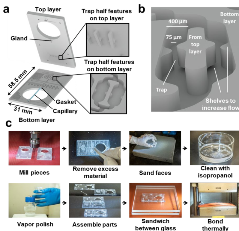
870 Figure 3 | Scalable manufacturing of the Islet on a Chip. a. Exploded view of the islet chip drawing in Figure 1b to show integration of the glass capillary and trap features on each layer before bonding. b. Angled, zoomed view of 875 two adjacent islet traps in the islet chip drawing in Figure 1b to visualize channel and trap detail. Middle island between each pair of channels protrudes from the bottom surface of the top layer and fits into the channel to complete the trap during bonding. A small opening above or below each wall in the traps was designed to increase flow through the traps. c. Photographs of steps in chip fabrication. First, chip features are milled into polycarbonate and excess material is removed. Layers are then sanded, cleaned, and vapor polished. Finally, the capillary is assembled between polished layers and bonded together.
