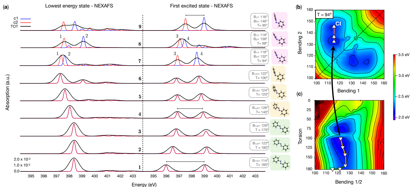
Fig. 6 (a) Lowest energy state and first excited state
