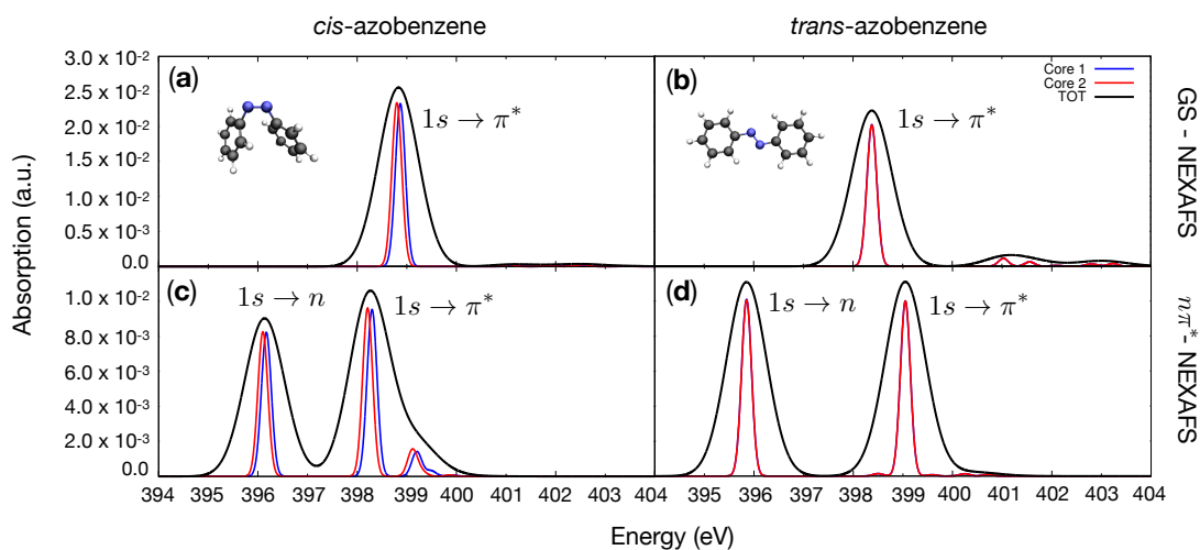
Fig. 2 NEXAFS spectra for cis -azobenzene (a,c) and trans -azobenzene (b,d). Color spectra are obtained with a gaussian broadening of 0.1 eV and correspond to exciting cores c1 (blue) and c2 (red, see Figure 1 for notation). The black spectrum represents the sum of the individual core spectra with a broadening of 0.4 eV. The molecular structure is also reported in the inset of (a) and (b). (a) and (b) show GS-NEXAFS, (c) and (d) show n\pi^* -NEXAFS of both species.
