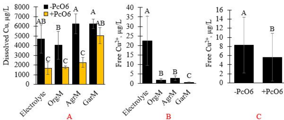
Fig. 4. Dissolved Cu (A) as affected by the interaction of RS and PcO6 and free Cu 2+ as affected by RS (B) and Pseudomonas chlororaphis O6 ( PcO6 ) (C) in planted samples with CuO NPs. The error bars show 95% confidence intervals (n = 6 (A), 12 (B), or 24 (C) per bar) to illustrate the spread of data, but do not determine significant differences. Bars with differing letters (A, B, etc.) are statistically different (p < 0.05) by Tukey's Honestly Significant Difference (A, B) or Student's t-test (C) after two-way ANOVA. Free Cu 2+ required a logarithmic transformation to maintain normal distributions of the residuals. When CuO NPs were not included, the RSs had an average of 50.6 ± 11.4 µg/L dissolved Cu and 0.30 ± 0.09 µg/L free Cu 2+ (95% confidence intervals).
