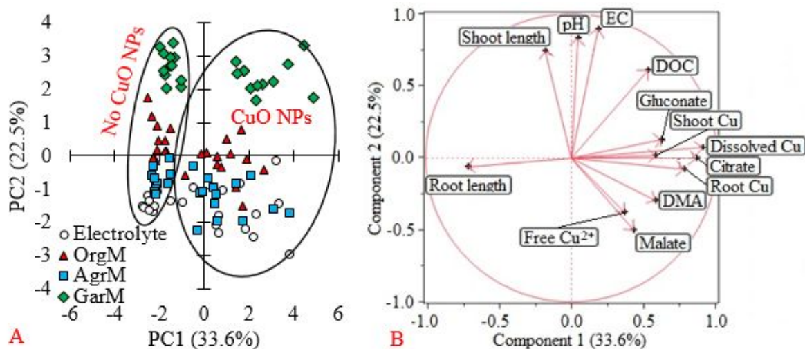
Fig. 5 Principal components analysis score plot (A) and loading plot (B) of all planted samples in study with and without Pseudomonas chlororaphis O6 ( PcO6 ). Score plot values for PcO6 samples were imputed by JMP. Variables included (13) were gluconate, malate, citrate, DMA, dissolved organic carbon (DOC), pH, electrical conductivity (EC), dissolved Cu after centrifugation, free \text{Cu}^{2+} , root Cu, shoot Cu, root length, and shoot length. Fulvic and humic acids were not included in the principal components analysis because they were only measured in the SPWs and not the RSs. PC = principal component.
