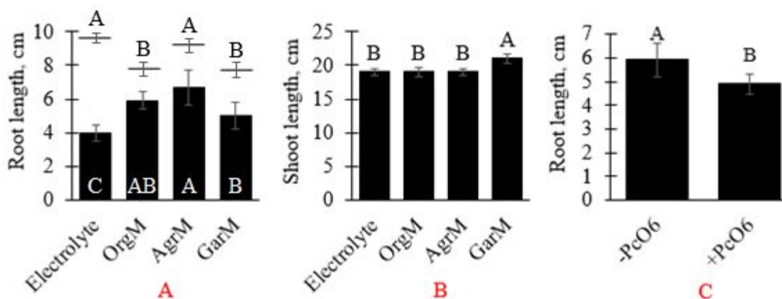
Fig. 2. Root length (A) and shoot length (B) as affected by RS, and root length as affected by Pseudomonas chlororaphis O6 ( PcO6 ) (C) in the presence of CuO NPs (100 mg Cu/kg). Shoot length was not affected by PcO6 and is not shown. The error bars show 95% confidence intervals ( n = 12 per bar in A, B and 24 per bar in C) to illustrate the spread of data, but do not determine significant differences. Bars with differing letters (A, B, etc.) are statistically different ( p < 0.05 ) by Tukey's Honestly Significant Difference or Student's t-test after two-way ANOVA. The horizontal bars in graph A show the root length of the non-CuO treated wheat. In graph A, the black letters only apply to horizontal bars, and the white letters only apply to vertical bars; there is no equivalency between the black and white letters.
