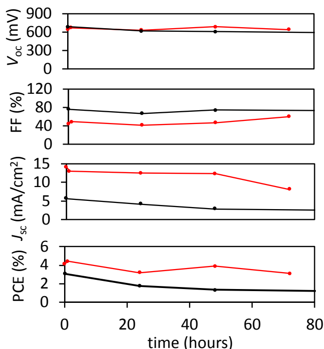
Figure 6. Stability curves for [\text{Cu}(1)]^{2+/1+} -PEDOT (black lines) and [\text{Cu}(2)]^{2+/1+} -Pt (red lines).
