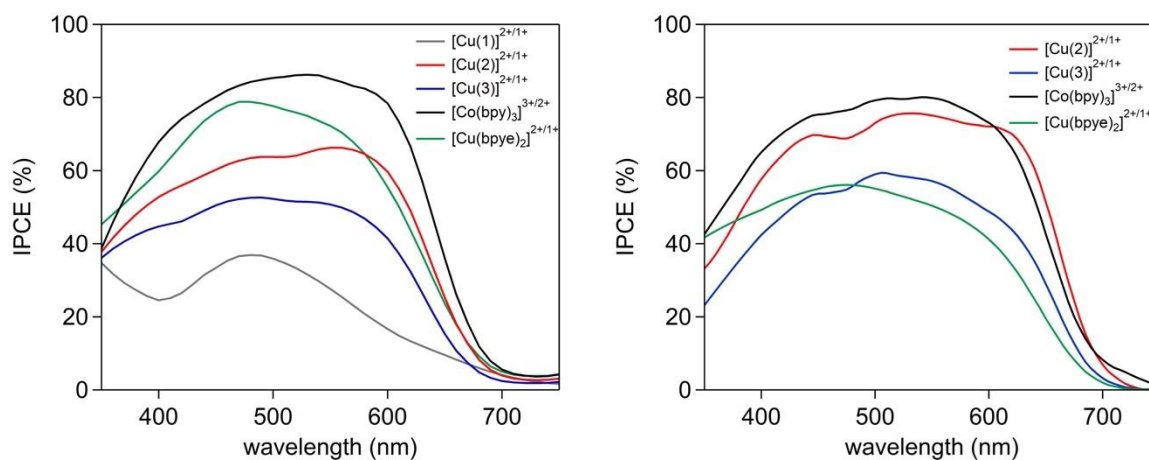
Figure 5. IPCE curves of DSC devices fabricated with PEDOT counter electrodes (left) or Pt counter electrodes (right) using Cu and Co RSs as specified with dye Y123 .
