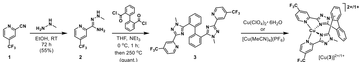
Scheme 1. Synthesis of the \text{CF}_3 -substituted biphenyl-based copper(II/I) redox shuttles.
