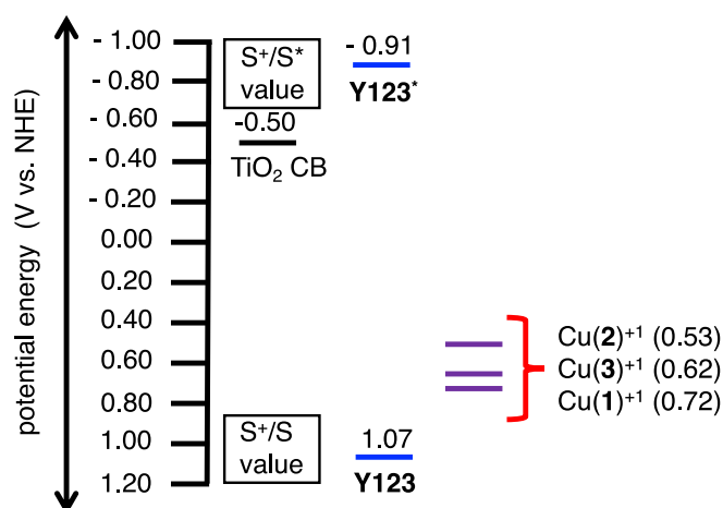
Figure 4. Energy level diagram for Y123 , [Cu(1)] 2+/1+ , [Cu(2)] 2+/1+ , and [Cu(3)] 2+/1+ . The TiO 2 conduction band (CB) is taken as -0.50 V vs. NHE in MeCN as is generally approximated in the field. 59-61
