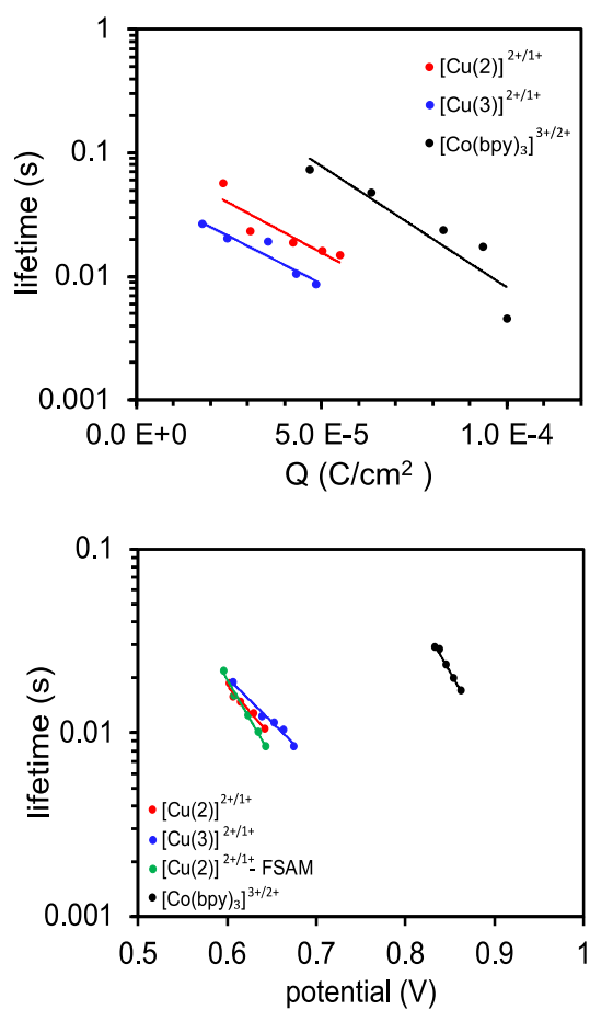
Figure 8. A plot of electron lifetime versus capacitance (top) and a plot of electron lifetime versus open-circuit voltage from SMPVT (bottom) with DSC devices based on Cu and Co RSs with Pt electrodes.
