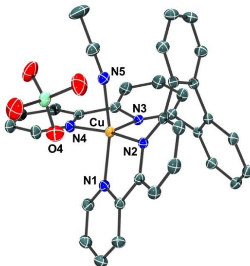
Figure 3. Crystal structure of [\text{Cu}(1)(\text{MeCN})](\text{ClO}_4)_2 with thermal ellipsoids rendered at 50% probability level. Hydrogen atoms have been omitted for clarity. One of the two perchlorate anions is shown due to its weak interaction with the Cu(II) metal center (Cu---O4 distance = 2.9033(12) Å).
