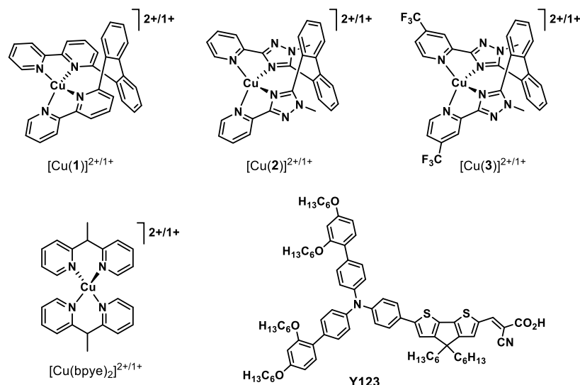
Figure 2. Structures of [\text{Cu}(\mathbf{1})]^{2+/1+} , [\text{Cu}(\mathbf{2})]^{2+/1+} , [\text{Cu}(\mathbf{3})]^{2+/1+} , [\text{Cu}(\text{bpye})_2]^{2+/1+} , and Y123 .
