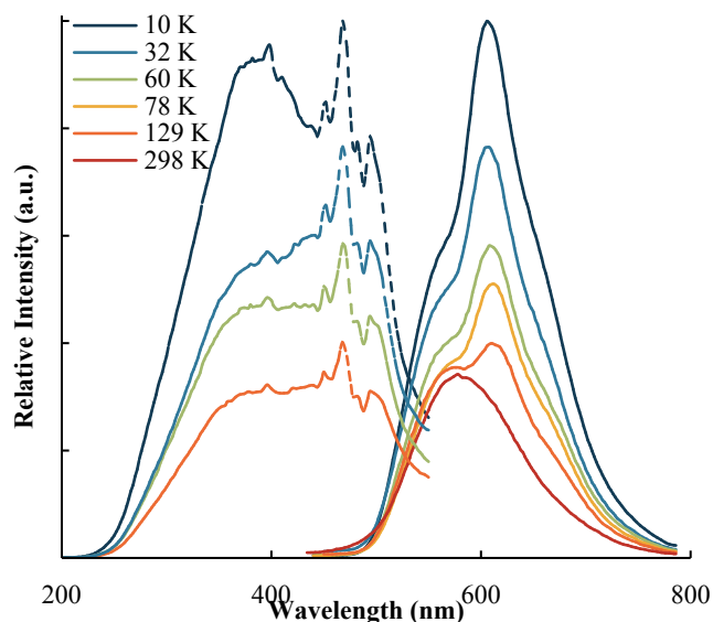
Fig. 5. Luminescence spectra of Au heli-viologen between 10 K and 298 K. Excitation (dashed) and emission (solid).
