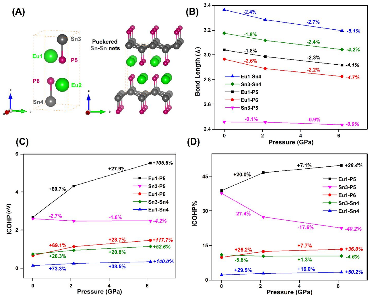
FIG. 1. (A). (Left) Crystal structure of EuSnP (green, grey, and red balls represent Eu, Sn and P, respectively). (Right) Puckerd Sn-Sn nets in EuSnP. (B). Trend plot for typical bond lengths in EuSnP under pressures. (C). Integrated Crystal Orbital Hamiltonian Population (ICOHP) trend under pressures for critical atomic interactions. (D). Percentage of ICOHP changes with pressure in EuSnP.
