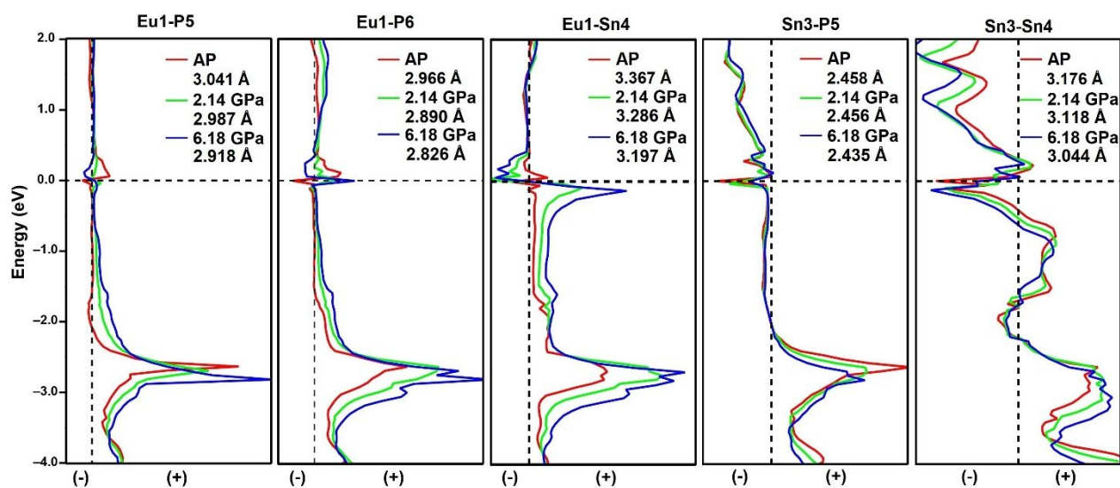
FIG. 2. Crystal Orbital Hamiltonian Population (COHP) calculation for atomic interactions in EuSnP under various pressures where (-) indicates anti-bonding interaction and (+) shows bonding interaction.
