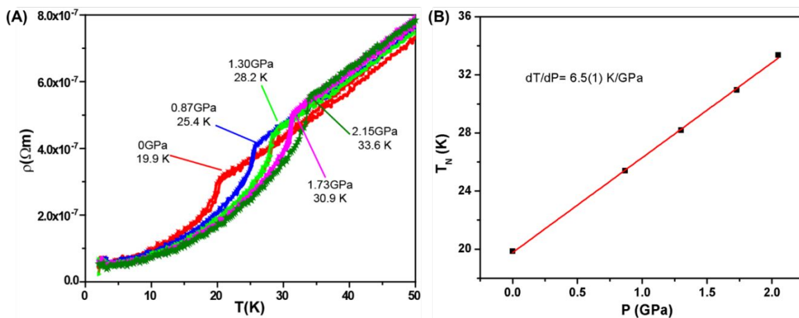
FIG. 3. (A) Temperature dependence of resistivity \rho(T) at various pressures up to 2.15 GPa with magnified temperature ranging from 2 to 50 K. (B) Pressure-dependent magnetic ordering transition temperatures with dT/dP = 6.5(1) K/GPa with R^2 = 0.999 .
