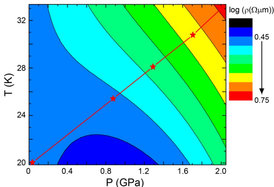
FIG. 4. Contour map in the temperature-pressure (T-P) plane for resistivity in EuSnP. The color bars at the side of the map represent the magnitude of the resistivity. The stars represent the transition temperatures at different pressures. ( 0 \text{ GPa} < P < 2.15 \text{ GPa} and 19.9 \text{ K} < T < 33.6 \text{ K} )
