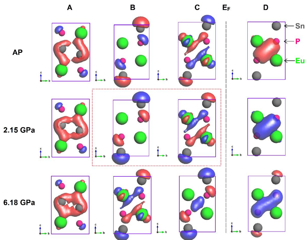
FIG. 5. Molecular Orbitals (MOs) of EuSnP under different pressures. Column A: MO #17 when moving origin from (0,0,0) to (\frac{1}{2}, \frac{1}{2}, \frac{1}{2}) ; Column B: MO #17; Column C: MO of orbital #18 (Highest occupied molecular orbital (HOMO)); Column D: MO of orbital #19 (Lowest unoccupied molecular orbital (LUMO)). Green, grey and pink balls represent Eu, Sn and P atoms, respectively. Red dashed line indicates degeneracy.
