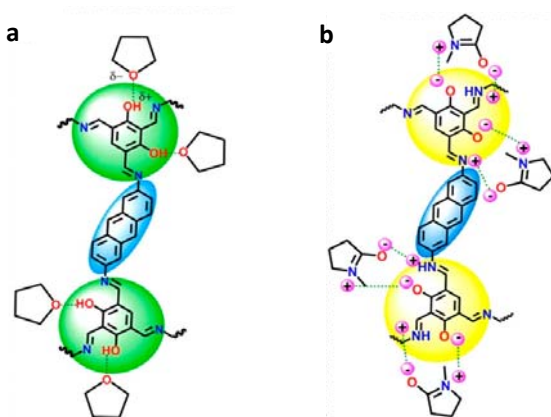
Fig. 7 (a) Stabilization of the enol-form due to hydrogen bonding by THF. (b) Stabilization of the intermediate keto-enol form by the polarized NMP. Adapted with permission from J. Am. Chem. Soc. 2018 , 140 , 13367. Copyright 2018 American Chemical Society.
