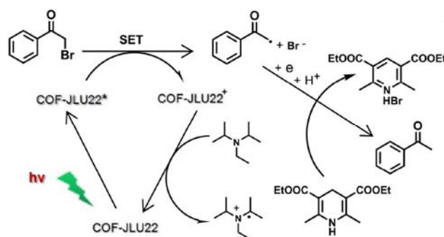
Fig. 29 Proposed mechanistic representation of the COF-JLU22 catalyzed photoreductive dehalogenation. Adapted with permission from Appl. Catal. B: Environ. 2019, 245, 334-342.
