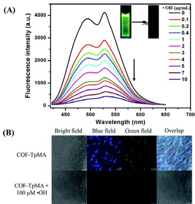
Fig. 24 (a) Fluorescence quenching of COF-TpMA upon the addition of \cdot OH. (b) Confocal laser scanning microscopy images of BHK cells treated with COF-TpMA (top) and pretreated with COF-TpMA and then treated with \cdot OH (bottom). Scale bar = 10 \mu m. Reproduced from Chem. Commun. , 2019 , 55 , 167-170, with permission from the Royal Society of Chemistry.
