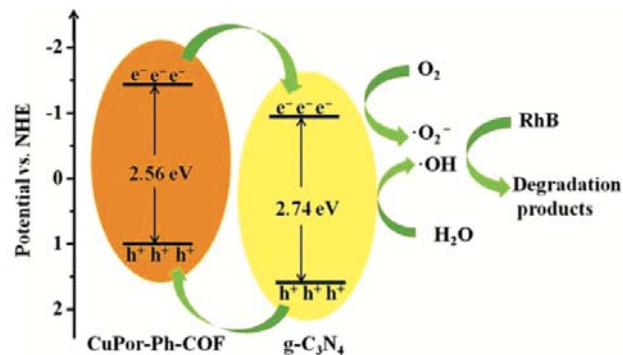
Fig. 31 Proposed mechanism for the photocatalytic degradation of rhodamine B by CuPor-Ph-COF/ g\text{-C}_3\text{N}_4 hybrid composite. Reproduced from Dalton T. 2019, 48, 14989-14995, with permission from the Royal Society of Chemistry.
