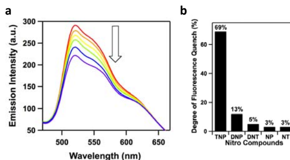
Fig. 15 (a) Fluorescence quenching of Py-Azine COF in MeCN (0.01 mg/mL) upon exposure to TNP vapors for various times (0-70 min). (b) Degree of fluorescence quenching after the addition of various nitro compounds (70 ppm). Adapted with permission from J. Am. Chem. Soc. 2013, 135, 17310-17313. Copyright 2013 American Chemical Society.
