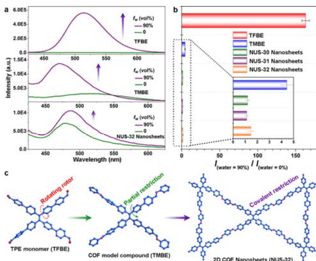
Fig. 9 (a) Fluorescence spectra ( \lambda_{exc} = 365 nm) of TFBE, TMBE, and NUS-32 in dry solvent or 90% water fractions. (b) Relative fluorescence intensities of TFBE, TMBE, and NUS-32 in solvent/water mixtures compared to dry solvent [ I_{(water = 90\%)} / I_{(water = 0\%)} ]. (c) Representation of the increasing restriction of AIE molecular rotor from monomer (TFBE) to COF model compound (TMBE) to 2D COF nanosheets (NUS-32). Reprinted with permission from Chemistry of Materials , 2019, 31, 146-160. Copyright 2019 American Chemical Society.
