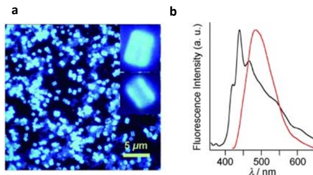
Fig. 10 (a) Fluorescence microscopic image of PPy-COF (the inset depicts an enlarged image of individual cubes). (b) Normalized fluorescence spectra ( \lambda_{exc} = 414 nm, 25 °C) of PDBA (black curve) and PPy-COF (red curve). Adapted with permission from Angew. Chem. Int. Ed. , 2009, 48, 5439-5442.
