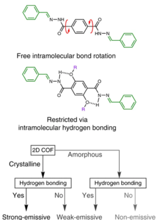
Fig. 14 Free intramolecular rotation in the amorphous solid state makes it non-emissive. (b) Intramolecular hydrogen bonding restricts rotation, causing enhanced emission in the UV to violet region. (c) Flow chart depicting the strategy to achieve strong solid state emission in 2D COFs. Adapted with permission from Nat. Commun. , 2018, 9, 233.
