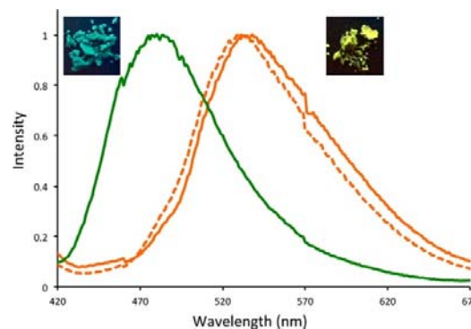
Fig. 12 Normalized emission spectra of Py-DBACOF 1 (orange, \lambda_{\text{ex}} = 350 \text{ nm} ), Py-DBA-COF 2 (green, \lambda_{\text{ex}} = 365 \text{ nm} ), and Py-MV-DBA-COF (dashed orange, \lambda_{\text{ex}} = 350 \text{ nm} ). Photographs of the fluorescent solids were taken using a hand-held UV-lamp at 365 nm. Reprinted with permission from J. Am. Chem. Soc. 2016, 138, 10120-10123. Copyright 2016 American Chemical Society.
