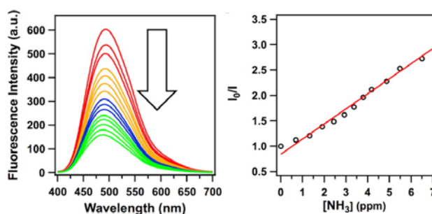
Fig. 22 (a) Fluorescence quenching of TPE-Ph COF upon the addition of ammonia. (b) Stern-Volmer plot of the ammonia driven fluorescence quenching of TPE-Ph COF. Adapted with permission from J. Am. Chem. Soc. , 2016, 138, 5797-5800. Copyright 2016 American Chemical Society.
