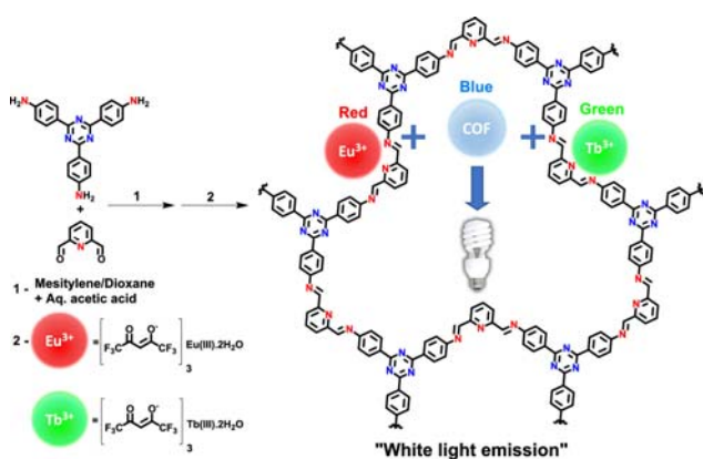
Fig. 33 Synthetic scheme for the formation of TTA-DFP COF and the subsequent grafting of lanthanides. Reprinted with permission from ACS Appl. Mater. Inter. , 2019, 11, 27343-27352. Copyright 2019 American Chemical Society.
