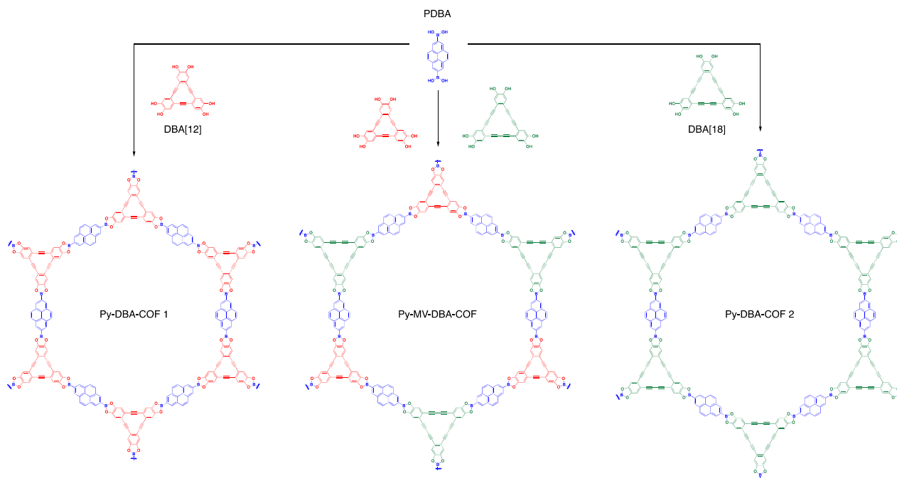
Fig. 11 Synthesis of Py-DBA-COF 1, Py-MV-DBA-COF, and Py-DBA-COF 2.
