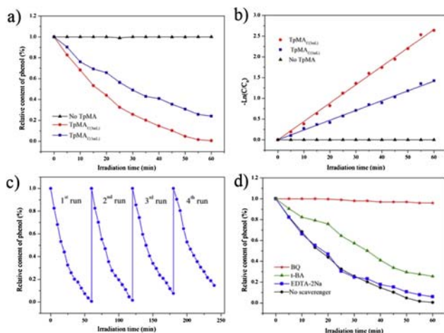
Fig. 30 (a) Visible light irradiated photocatalytic degradation of phenol. (b) Linear simulation -\ln(C/C_0)=kt of the kinetic curves. (c) Recyclability of TpMA. (d) Scavenger effects on the photo-degradation of phenol. Reprinted with permission from J. Hazard. Mater. , 2019, 369, 494-502.
