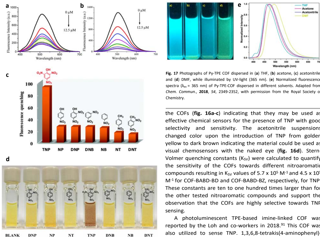
Fig. 16 Fluorescence spectra ( \lambda_{\text{ex}} = 370 nm) of (a) COF-BABD-DB and (b) COF-BABD-BZ dispersed in MeCN with the addition of varying amounts of TNP. (c) Fluorescence quenching (%) of COF-BABD-BZ with different nitroaromatics (12.5 \mu\text{M} ). (d) Photographs of COF-BABD-DB dispersed in MeCN with the addition of various nitroaromatics (4.0 \mu\text{M} ). Adapted from Chem. Commun. , 2018, 54, 2308-2311, with permission from the Royal Society of Chemistry.
