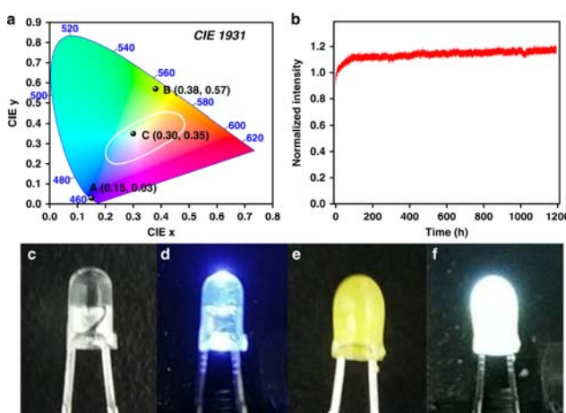
Fig. 35 (a) CIE diagram of blue LED (A), 3D-TPE-COF (B), and COF-coated LED (C). (b) Normalized emission intensity for the COF-coated LED over 1200 h, at 2 mA. Photographs of reference blue LED when off (c) and on (d), COF-coated LED when off (e) and on (f). Reprinted with permission from Nat. Commun. , 2018, 9, 5234.
