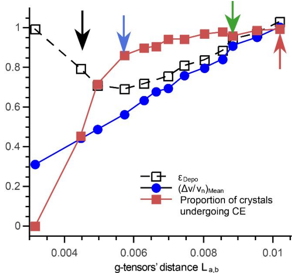
Fig. 4: Blue circles, mean value of (|\Delta\nu|/\nu_n)_{\text{Mean}} , red squares proportion of orientation undergoing CE under MAS, black squares and dotted line, \epsilon_{\text{Depo}} plotted against the g-tensors' distance L_{a,b} . Black, red, green and blue arrows correspond to the four illustrative orientations.
