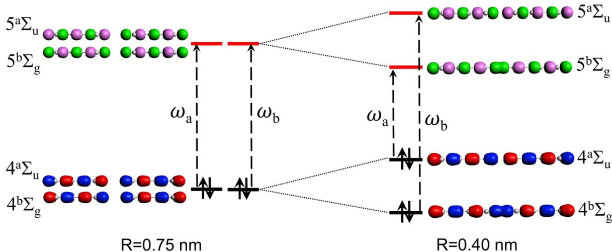
Figure 3. Schematics of the interaction picture between occupied and unoccupied levels of Ag_8 atomic wire dimers with changing gap distance. At 0.75 nm, there is little overlap between monomeric orbitals, which results in nearly degenerate 4^a\Sigma_u and 4^b\Sigma_g levels for HOMO and 5^b\Sigma_g and 5^a\Sigma_u levels for LUMO. This near-degeneracy is broken as a result of significant overlap for shorter distances as shown for 0.40 nm. The dipole-allowed transitions ( 4^a\Sigma_u \rightarrow 5^b\Sigma_g and 4^b\Sigma_g \rightarrow 5^a\Sigma_u ) are shown with dashed lines.
