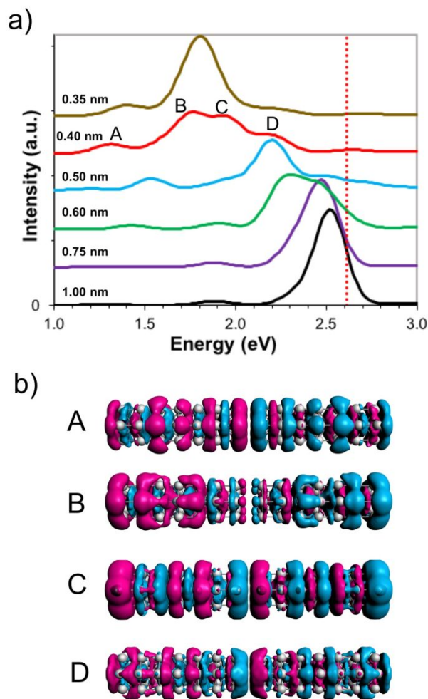
Figure 6. a) Calculated spectra with PBE/DZ level of theory for \text{Ag}_{41}^{-1} nanorod dimers at gap distances between 1.00 and 0.35 nm and b) calculated TFDs for the selected excited states for the dimer with gap distance of 0.40 nm. TFDs correspond to the excited states at 1.32, 1.76, 1.96 and 2.21 eV from top to bottom respectively.
