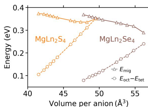
Figure 4. Comparing the Mg 2+ migration energy, E_{\text{mig}} , to the difference in octahedral and tetrahedral energies, E_{\text{oct}} - E_{\text{tet}} as a function of the calculated volume per anion in the pristine structures.
