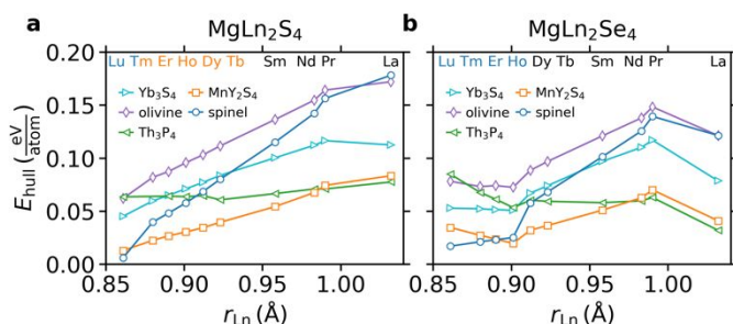
Figure 5. Stability with respect to competing phases, E_{hull} , for each sulphide ( a ) and selenide ( b ) in a variety of crystal structures common to AB_2X_4 -type compounds. The colour of each element at
