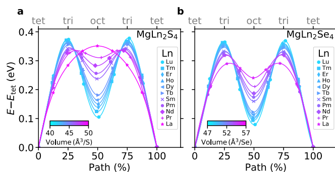
Figure 3. Energy profiles for vacancy-mediated Mg 2+ migration in sulphides (a) and selenides (b). Energy is shown relative to the tetrahedral Mg state ( E - E_{\text{tet}} ). The colourbar provides the volume per anion of the pristine structure.
