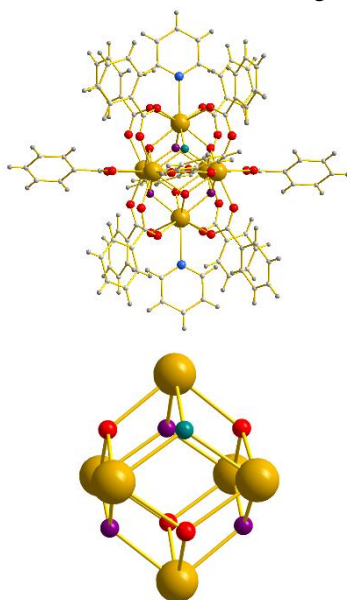
Fig. 3 (a) The complete structure of 2 , and (b) the [Ce 6 O 4 (OH) 3 F] core with only one set of disorder positions shown for clarity. Colour code: Ce IV gold, O red, OH purple, F teal, N blue, C and H grey.
