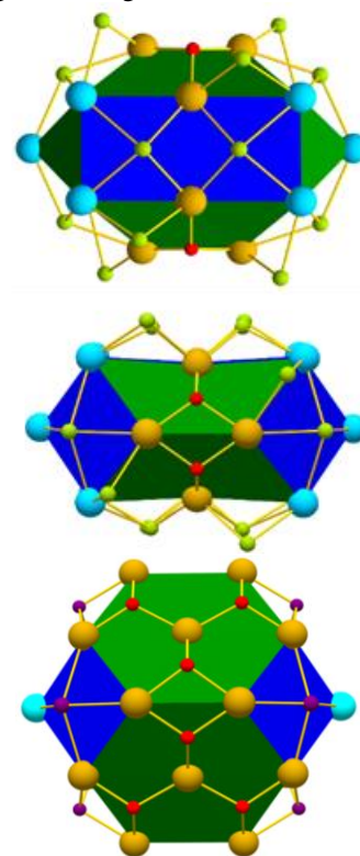
Fig. 2 (a, b) The Ce 20 anion of 1 from two perpendicular viewpoints, with the benzoate ligands omitted for clarity. Facets are colour coded: (100) blue, (111) green. The μ 4 -Cl - ions bridge (100) facets, whereas μ 2 -Cl - ions bridge edges linking (111)(100) facets. (c) The Ce 24 cluster from the same viewpoint as in (b), and with benzoate and py ligands omitted, Colour code: Ce IV gold, Ce III sky blue, O red, OH - purple, Cl green.
