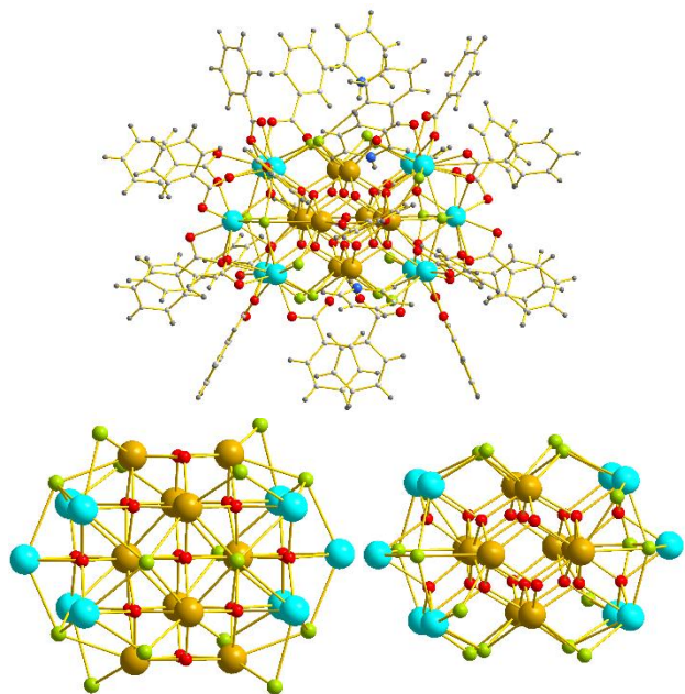
Fig. 1 (a) The complete structure of the anion of 1 , and (b) its Ce 20 O 18 Cl 16 core from two viewpoints differing by rotation about the horizontal axis. Colour code: Ce IV gold, Ce III sky blue, O red, Cl green, N blue, C light grey, H dark grey.
