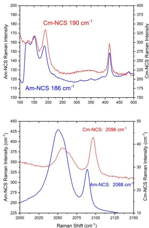
Figure 2 Raman spectra of the americium and curium thiocyanate complexes in the regions of the metal-nitrogen stretch as well as the N≡C stretch at higher frequency.
