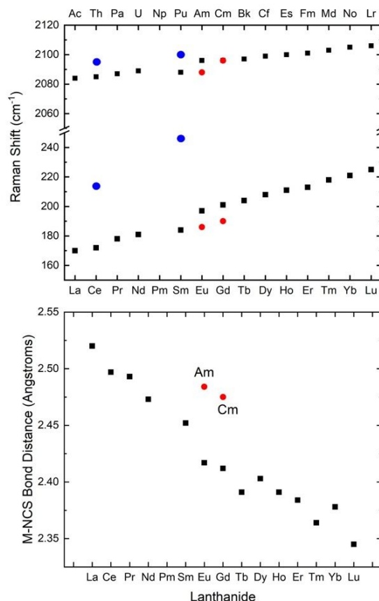
Figure 3 The observed Raman frequencies for the actinide and lanthanide thiocyanate complexes, top panel. The lanthanide frequencies are represented by the black squares, the Am(III) and Cm(III) frequencies are the red dots, Th(IV) and Pu(IV) in the blue dots. 12 The higher frequency vibrations ( 2080\text{--}2100\text{ cm}^{-1} ) are associated with the N≡C vibrations of NCS, while the lower frequencies ( 160\text{--}250\text{ cm}^{-1} ) arise from the M-N vibrations. The lower panel highlights the trend in bond distances in the data.
