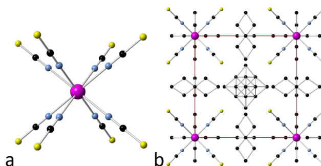
Figure 1 a. The coordination environment of the trivalent lanthanide and actinide thiocyanate complexes, the metal is shown in magenta, nitrogen in blue and carbon in black and sulfur in yellow. The thiocyanates are 7/8th occupied making the metals seven coordinate, An(NCS)_7^{4-} . b. Packing diagram for the Pm3m phases with the tetraethylammonium groups shown.
