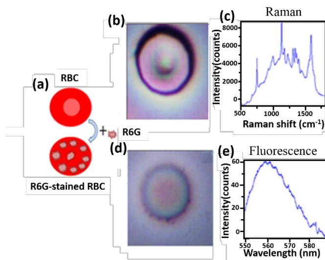
Fig 1. (a) Schematic of the R6G-stained RBC preparation. Optical microscope images of RBC, 8 \times 8 \mu\text{m} (b) and R6G-stained RBC, 10 \times 10 \mu\text{m} (d) and the corresponding resonance Raman (c) and fluorescence (e) spectra. The spectrum of RBC is dominated by the resonance Raman signal of Hb, whereas the spectrum of R6G-stained RBC is dominated by the fluorescence of R6G (at low laser power).
