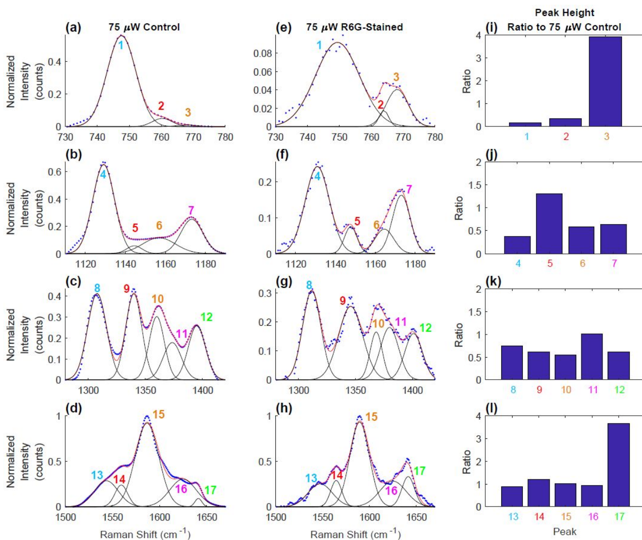
Fig. 5. Raman spectra of the dried fresh unstained control RBC (a-d) and dried fresh R6G-stained RBC (e-h) normalized to the intensity of the 1590 cm -1 band at 75 μW laser power show the absence of the significant staining effects on RBC. The observed strong intensities of bands 3 and 17 are attributed to the resonance Raman signals of R6G. Solid black lines are the Gaussian fits of the selected marked bands and solid red lines are the combined fits. (i-l) Peak height ratios of the normalized peak intensities of the dried fresh R6G-stained RBC to the normalized peak intensities of the unstained dried fresh RBC (control) at 75 μW.
