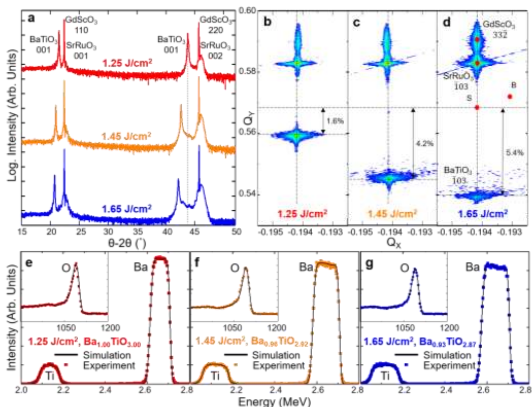
Fig. 1 (a) \theta -2 \theta X-ray diffraction scans of the \text{Ba}_{1-x}\text{TiO}_y/\text{SrRuO}_3/\text{GdScO}_3 (110) heterostructures grown at laser fluences of (top, red) 1.25 \text{J}/\text{cm}^2 , (middle, orange) 1.45 \text{J}/\text{cm}^2 , and (bottom, blue) 1.65 \text{J}/\text{cm}^2 . Off-axis reciprocal space mapping studies about the \bar{1}03 - and 3\bar{3}\bar{2} -diffraction conditions of the film and substrate, respectively, with the heterostructures grown at laser fluences of (b) 1.25 \text{J}/\text{cm}^2 , (c) 1.45 \text{J}/\text{cm}^2 , and (d) 1.65 \text{J}/\text{cm}^2 . Rutherford backscattering spectra with a zoom-in about the oxygen resonance peak (inset) for heterostructures grown at laser fluences of (e) 1.25 \text{J}/\text{cm}^2 , (f) 1.45 \text{J}/\text{cm}^2 , and (g) 1.65 \text{J}/\text{cm}^2 .
