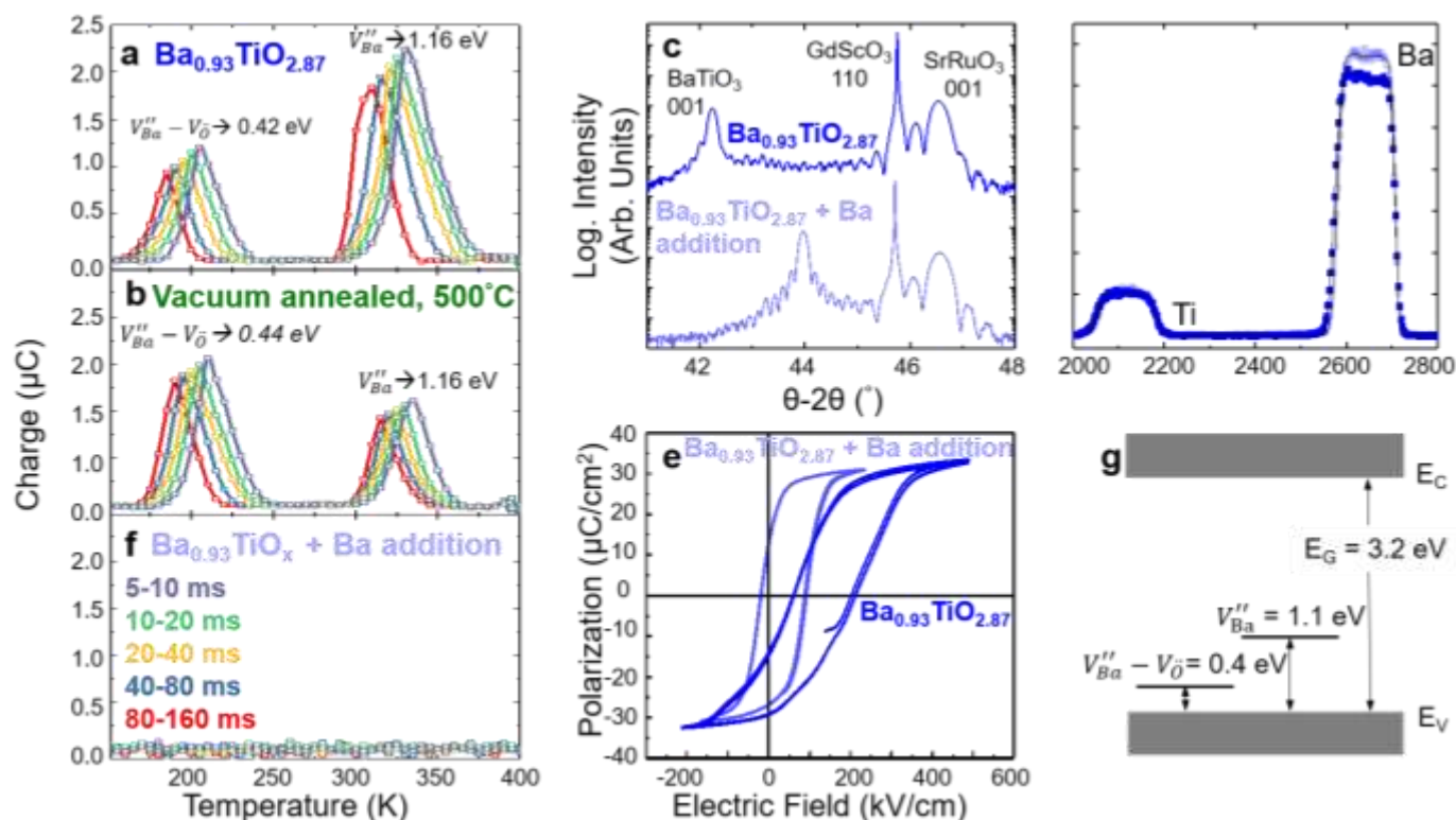
Fig. 5 Deep-level transient spectroscopy data for (a) an as-grown \text{Ba}_{0.93}\text{TiO}_{2.87} heterostructure, (b) the same film after vacuum annealing at 500^\circ\text{C} , and (f) the same after barium addition via the CVD-like process. (c) \theta - 2\theta X-ray diffraction scans of the \text{Ba}_{0.93}\text{TiO}_{2.87} heterostructure in the (top) as-grown state and (bottom) following barium addition via CVD-like process. (d) Rutherford backscattering spectra and (e) polarization-electric field hysteresis loops for the \text{Ba}_{0.93}\text{TiO}_{2.87} heterostructure in the as-grown state and following barium addition via the CVD-like process. (g) Schematic of the defect state energies present within the \text{Ba}_{1-x}\text{TiO}_y films wherein E_G is the band gap of \text{BaTiO}_3 .
