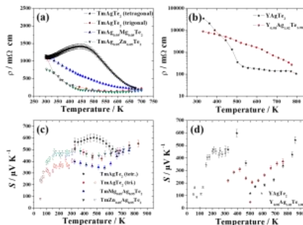
dependent Seebeck coefficient calculated from the crystal Figure 6: Experimental electrical resistivity of (a) TmAgTe 2 and (b) YAgTe 2 compounds indicating semiconducting behavior. The experimental Seebeck coefficient of (c) TmAgTe 2 and (d) YAgTe 2 is high due to a low carrier concentration. For comparison with the parent compound high-temperature electrical properties of LT-TmAgTe 2 (tetr.) and HT-TmAgTe 2 (tri.) were taken from Zhu et al. [22]
