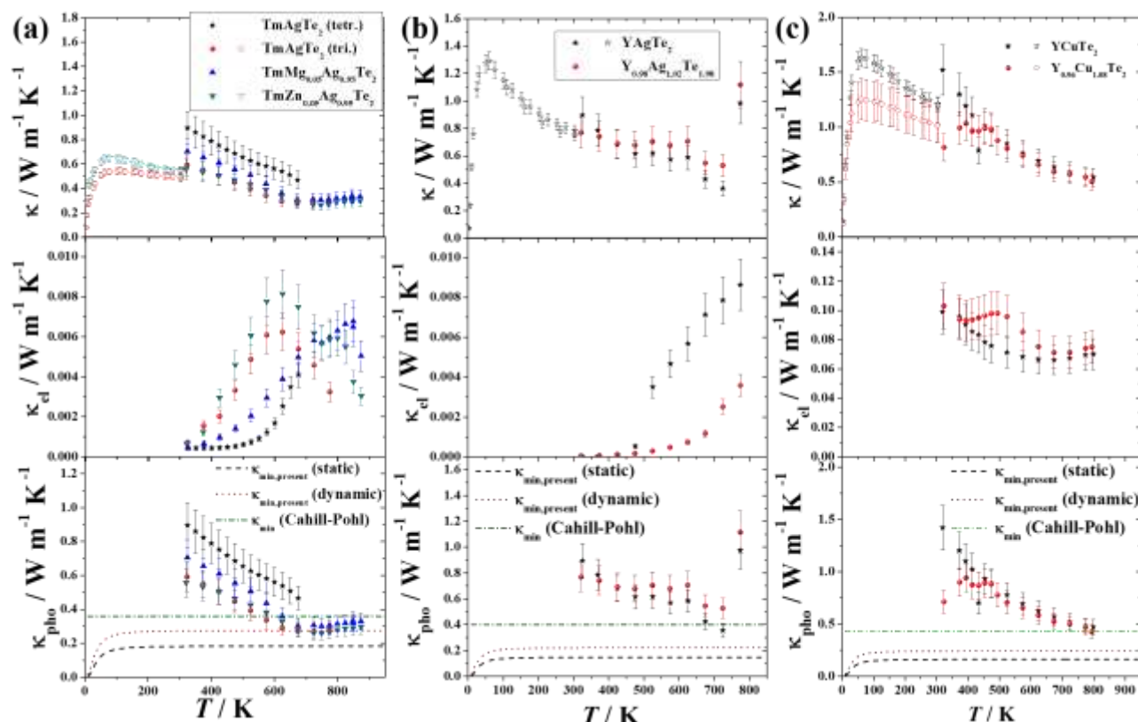
Figure 9: Total thermal conductivity, electronic and phononic contribution of (a) TmAgTe 2 , (b) YAgTe 2 , and (c) YCuTe 2 (including the corresponding doped compounds). The thermal conductivity of all parent compounds decreased below the Cahill and Pohl [38,39] minimum thermal conductivity limit ( \kappa_{min} ). The experimental thermal conductivity of HT-TmAgTe 2 approaches the dynamic limit ( i.e. , phonon mean free path is frequency-dependent) whereas the static limit ( i.e. , phonon mean free path is frequency-independent) underestimates the thermal conductivity. High-temperature thermal conductivity of the LT- and HT-phase of TmAgTe 2 was taken from reference [22] and the high-temperature thermal conductivity of YCuTe 2 and Y 0.96 Cu 1.08 Te 2 was taken from reference [23].
