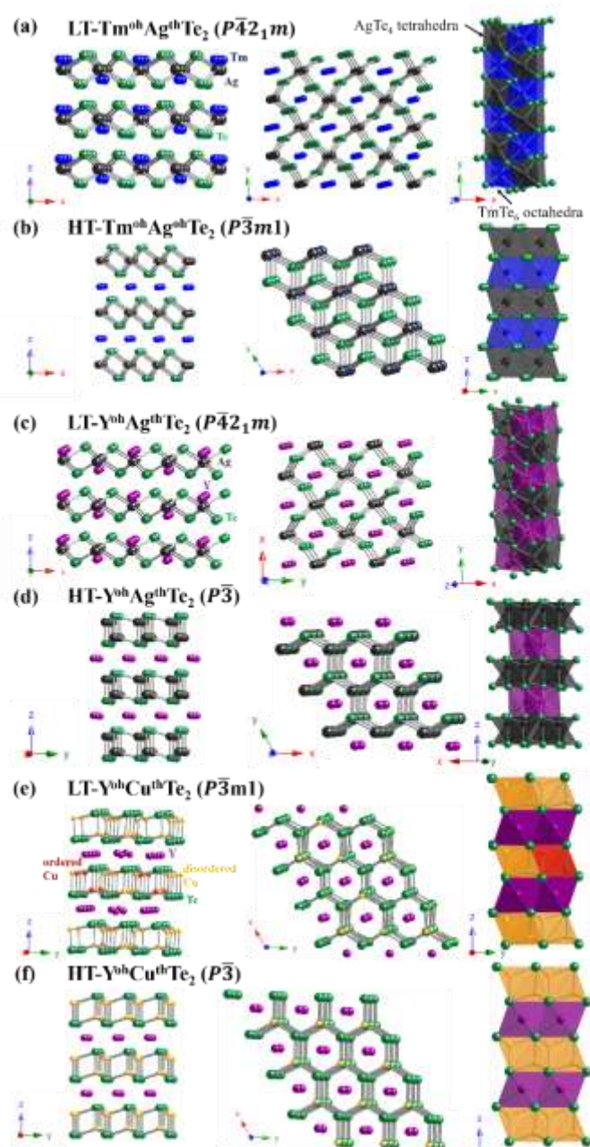
Figure 1: Crystal structures of (a) the LT phase ( P\bar{4}2_1m ) and (b) the HT phase ( P\bar{3}m1 ) of TmAgTe 2 , (c) the LT phase ( P\bar{4}2_1m ) and (d) the HT phase ( P\bar{3} ) of YAgTe 2 , and (e) the LT phase ( P\bar{3}m1 ) and (f) the HT phase ( P\bar{3} ) of YCuTe 2 (oh = octahedral interstices, th = tetrahedral interstices).
