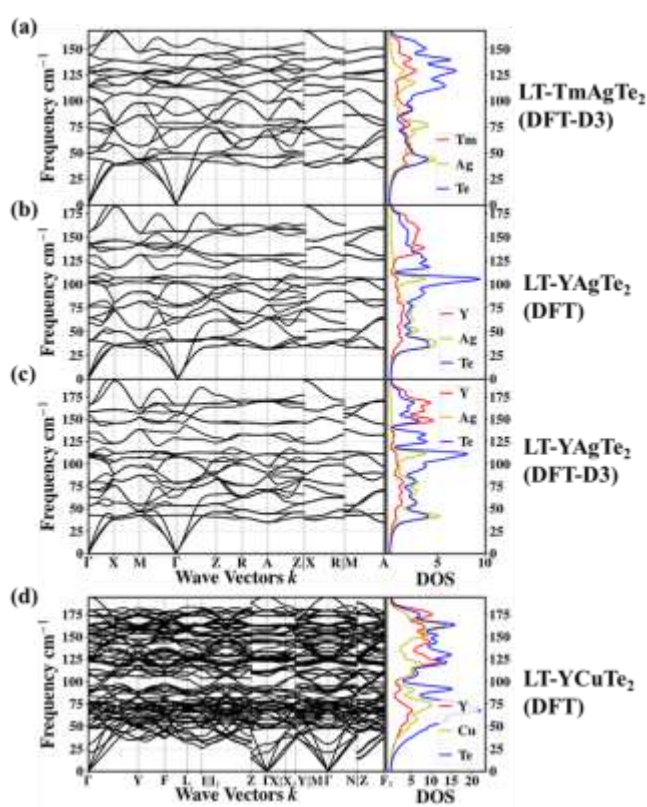
Figure 7: Computed phonon dispersion curves of (a) LT-TmAgTe 2 (DFT-D3), (b) LT-YAgTe 2 (DFT), (c) LT-YAgTe 2 (DFT-D3), and (d) the monoclinic phase of YCuTe 2 . The partial phonon DOS of the individual elements is provided to depict the contributions of the elements to the dispersions.
