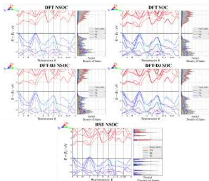
Figure 2: Electronic band structures of LT-TmAgTe 2 using PBE-GGA with and without the inclusion of spin-orbit coupling (SOC) and van der Waals interactions (DFT-D3) as well as using HSE06 without including spin-orbit coupling (NSOC). The degeneracy of the valence bands at the \Gamma points breaks due to SOC and/or DFT-D3. The different colors in the electronic band structure represent the contributions of different elements to the various band structures.
