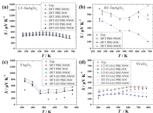
Figure 5: Computed and experimental Seebeck coefficient of (a) LT-TmAgTe 2 , (b) HT-TmAgTe 2 , (c) YAgTe 2 , and (d) YCuTe 2 . The carrier concentration and temperature for the calculations were taken from experiments. Experimental Seebeck coefficient for LT- and HT-TmAgTe 2 were taken from Zhu et al. [22] and for YCuTe 2 was taken from Aydemir et al. [23]
