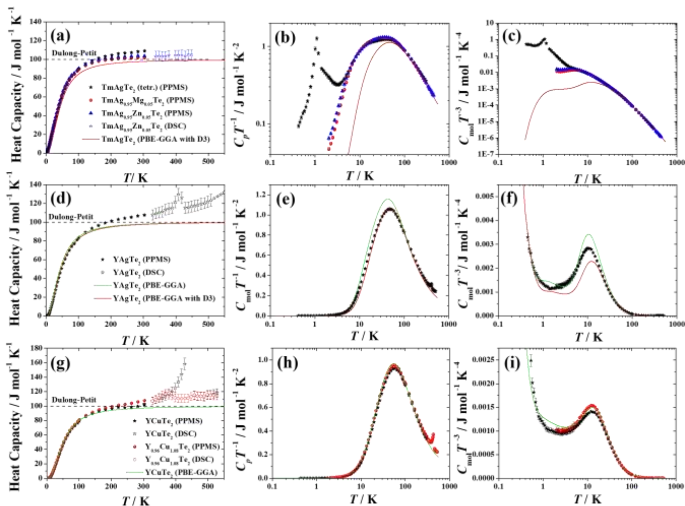
Figure 8: Comparison of computed and experimental heat capacity of (a-c) TmAgTe 2 , (d-f) YAgTe 2 , and (g-i) YCuTe 2 . The heat capacity was divided by T (to emphasize the intermediate-temperature range) and T^3 (to emphasize the low-temperature range). An overestimation of the computed heat capacity was observed without van der Waals forces whereas an underestimation was observed when van der Waals forces were included. High-temperature heat capacity of TmAgTe 2 and YCuTe 2 /Y 0.96 Cu 1.08 Te 2 were taken from Zhu et al. [22] and Aydemir et al. [23] respectively.
