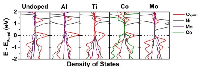
Figure 4: The partial density of states for the lowest E_{Ov}^F site and neighboring transition metals prior to oxygen removal. Analysis shows that Mo doping shifts the bonding states below the Fermi energy, and increases electron density below the Fermi energy, a potential source of anion stabilization.
