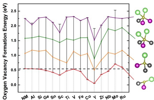
Figure 2: Distribution of oxygen vacancy formation energies, E_{Ov}^E , for each oxygen site for a full range of dopants. Representative bonding environments are indicated to reflect their relative E_{Ov}^E .
