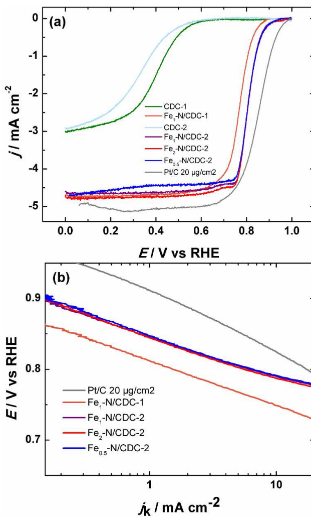
Figure 7. (a) ORR polarization curves (not corrected for iR) measured with RDE method for undoped CDCs, B_4C -derived and TiC-derived catalysts in O_2 -saturated 0.5 M H_2SO_4 . v = 10 \text{ mV s}^{-1} , \omega = 1600 \text{ rpm} . (b) Tafel plots calculated from the RDE data shown in (a). Catalyst loading = 803 \mu\text{g cm}^{-2} , except Pt/C ( 20 \mu\text{g}_{Pt} \text{ cm}^{-2} )
