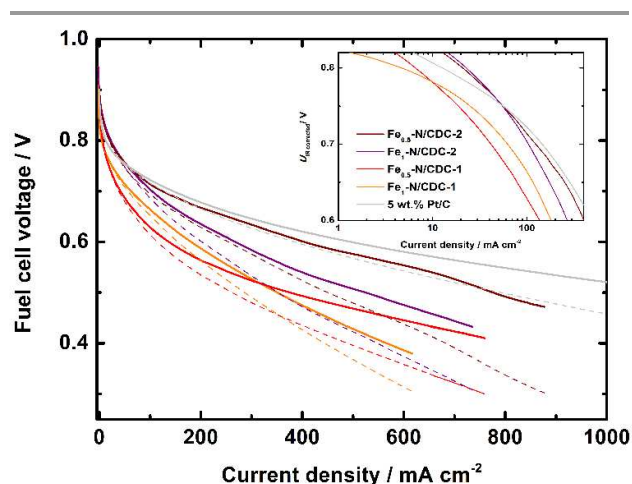
Figure 9. PEMFC polarization curves with cathodes comprising 4 mg cm -2 of Fe-N-C catalysts, as-measured (dashed curves) and after IR-correction (solid curves). The fuel cell temperature was 80 °C, pure O 2 and H 2 gases were humidified at 100% RH at cell temperature, the gas pressure was 1 bar. Inset: Tafel plots at high potential of IR-free polarization curves.
