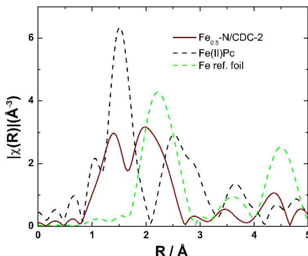
Figure 6. The FT-EXAFS of the sample \text{Fe}_{0.5}\text{N/CDC-2} , \text{Fe(II)Pc} , and iron reference foil (intensity reduced by a factor of 6 for the Fe foil, for comparison purpose).
