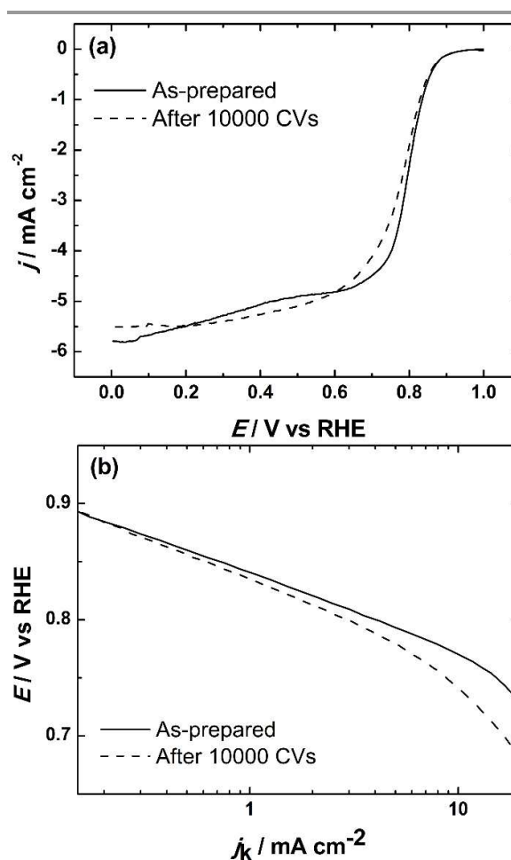
Figure 8. (a) ORR polarization curves of Fe 0.5 -N/CDC-2-modified GC electrodes in O 2 -saturated 0.5 M H 2 SO 4 before and after 10,000 CVs. v = 10 \text{ mV s}^{-1} , \omega = 1600 \text{ rpm} . (b) Tafel plots calculated from the RDE data shown in (a).
