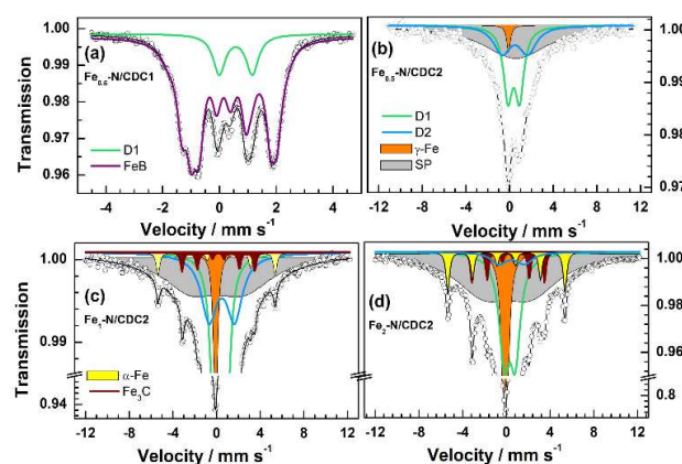
Figure 5. Room temperature ^{57}\text{Fe} Mössbauer spectra of (a) \text{Fe}_{0.5}\text{N/CDC-1} , (b) \text{Fe}_{0.5}\text{N/CDC-2} , (c) \text{Fe}_1\text{-N/CDC-2} , (d) \text{Fe}_2\text{-N/CDC-2} . For (c) and (d), note that the Y-axis scale is broken in order to improve the visibility of the low intensity components of magnetic Fe (sextets) and of the doublets.
