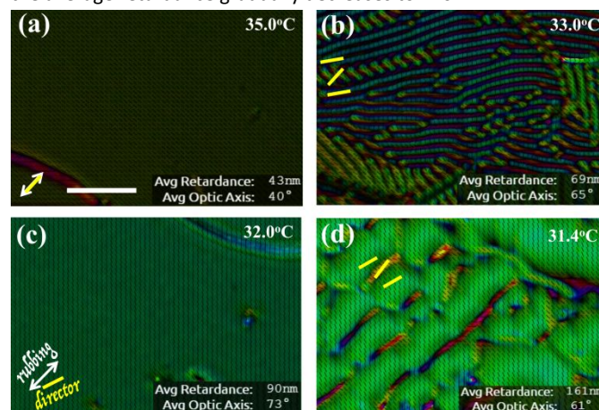
Figure 2: Phi-Viz images for a L = 4.7 \mu\text{m} film of KA(0.2)+2% ZLI811 at various temperatures. The dark lines are perpendicular to the LC director. (a): 35.0^\circ\text{C} , uniform texture in the N^* phase; (b): 33.0^\circ\text{C} , stripe domains with different orientations; (c): 32.0^\circ\text{C} , texture with uniform director with direction making 33^\circ with the rubbing direction; (d): 31.4^\circ\text{C} texture with stripes forming along the rubbing direction resembling the optical stripes typical of the N_{TB} phase. White bar shows 50 \mu\text{m} length. Insets at the bottom-right show the average retardance and average optical axis.
