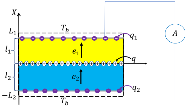
Fig. 4 Temperature difference applied to the two-film layered electret consisting of embedded charge q at the interface (Figure 1), and induced charges q_1 and q_2 at the upper and lower surfaces. Dashed lines shows the undeformed structure. L_1 and L_2 represent the reference thicknesses of layers and l_1 and l_2 are the thicknesses for the deformed structure.
