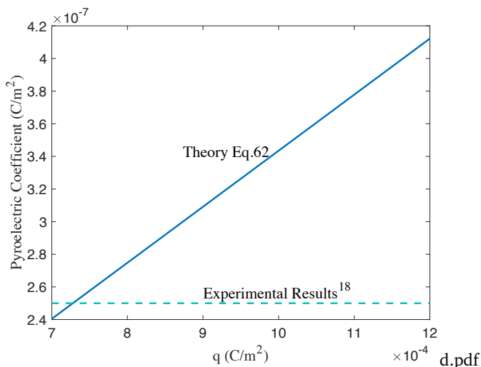
Fig. 8 Variation of pyroelectric coefficient for the porous electret shown in Figure 7 with respect to the charge density at the interface. Here, \epsilon_p = 2.2\epsilon_0 , H_p = 26\mu\text{m} , H_a = 44\mu\text{m} , T = 25^\circ\text{C} , and \Delta T = 10^\circ\text{C} .
