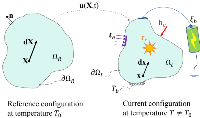
Fig. 3 Thermo-electro-mechanical system: \Omega_R and \Omega_t are the reference and spatial configurations of the system, and \partial\Omega_R and \partial\Omega_t are the according boundaries. \mathbf{X} and \mathbf{x} represent the position of the material in Lagrangian and Eulerian coordinates and \mathbf{n} is the unit outward vector. \mathbf{t}_e and h_e are the traction and heat flux applied to the system. T_0 is the initial temperature of the system and T_b corresponds to the temperature boundary condition. r_e is the heat source, \xi_b is the electrical potential, and \mathbf{u} is the displacement vector.
