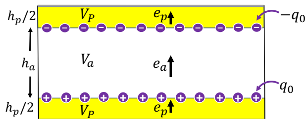
Fig. 7 A simplified model for the porous cellular polymer electret with opposite charges on the surfaces of voids.
