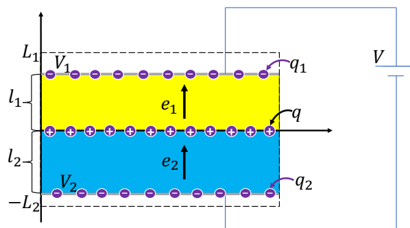
Fig. 10 Voltage difference applied to bilayer film structure with embedded charge q at the interface (Figure 1), and induced charges q_1 and q_2 at the upper and lower surfaces. Adiabatic boundary conditions are assumed. the dashed line shows the undeformed structure. L_1 and L_2 represent the reference thickness of each layer and l_1 and l_2 are the thicknesses of the deformed structure.
