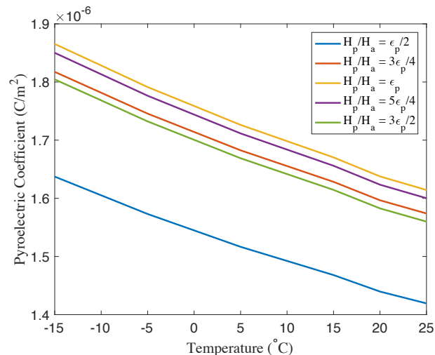
Fig. 9 Variation of pyroelectric coefficient with respect to temperature for the porous electret shown in Figure 7. The polymer is polyimide with \epsilon_p = 2.8\epsilon_0 45 , \alpha_p = 4 \times 10^{-5}/\text{K} 46 , q = 0.002\text{C}/\text{m}^2 , \Delta T = 10^\circ\text{C} .
