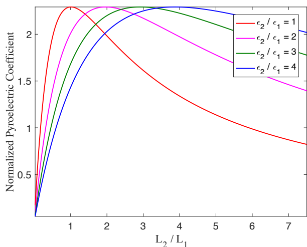
Fig. 6 Variation of pyroelectric coefficient normalized with respect to the experimental value of Bauer and co-workers 18 ( 2.5 \times 10^{-7}\text{C}/\text{m}^2\text{K} ) 17 for the electret shown in Figure 4. In that, \epsilon_1 = \epsilon_0 , \alpha_1 = 1.2 \times 10^{-3}\text{K}^{-1} , \alpha_2 = 4 \times 10^{-5}\text{K}^{-1} , L_1 = 70\mu\text{m} , q = 0.002\text{C}/\text{m}^2 , \Delta T = 10^\circ\text{C} , and both layers' elastic modulus is 1\text{MPa} .
