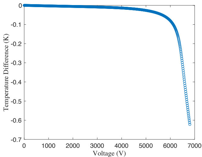
Fig. 12 Temperature difference with respect to the voltage applied to the system schematically shown in Figure 7. The electret is initially at room temperature, polymer is polypropylene with C_p = 1920 \text{J/KgK} , \rho_p = 904 \text{Kg/m}^3 , \alpha_p = 8 \times 10^{-5} \text{K}^{-1} , \mu_p = 400 \text{MPa} , E = 0.8 \text{MPa} , \varepsilon_p = 2.35\varepsilon_0 , H_p = 32 \mu\text{m} , H_a = 38 \mu\text{m} , \alpha_a = 3.4 \times 10^{-3} \text{K}^{-1} , C_a = 1000 \text{J/KgK} , \rho_a = 1.2 \text{Kg/m}^3 and the electric charge density at the interface is 0.001 \text{C/m}^2 .
