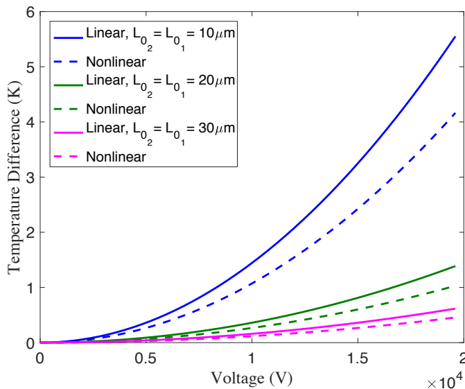
Fig. 11 Temperature difference with respect to the voltage applied to the system schematically shown in Figure 10. The materials are polypropylene and polyethylene at room temperature with material properties recorded in Table 2 and the electric charge density at the interface is 0.002C/m 2 .
