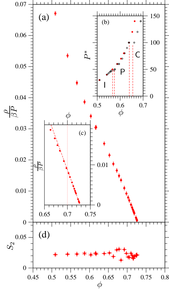
FIG. 12. (a) Inverse compressibility factor \frac{\rho}{\beta P} as a function of volume fraction \phi for lenses with \kappa \simeq 0.70 ; the upper inset (b) compares the dimensionless pressure P^* obtained on compression starting from the I fluid phase (filled circles) with that obtained on decompression starting from a densest-known orthorhombic configuration (empty circles), with the vertical dashed lines approximately delimitating equilibrium phase boundaries; the lower inset (c) zooms in on the high-volume-fraction region, with the dotted line indicating the value of \phi beyond which a free-volume-theory-inspired linear fit, the dashed line, was carried out. (d) Nematic order parameter S_2 as a function of volume fraction \phi .
