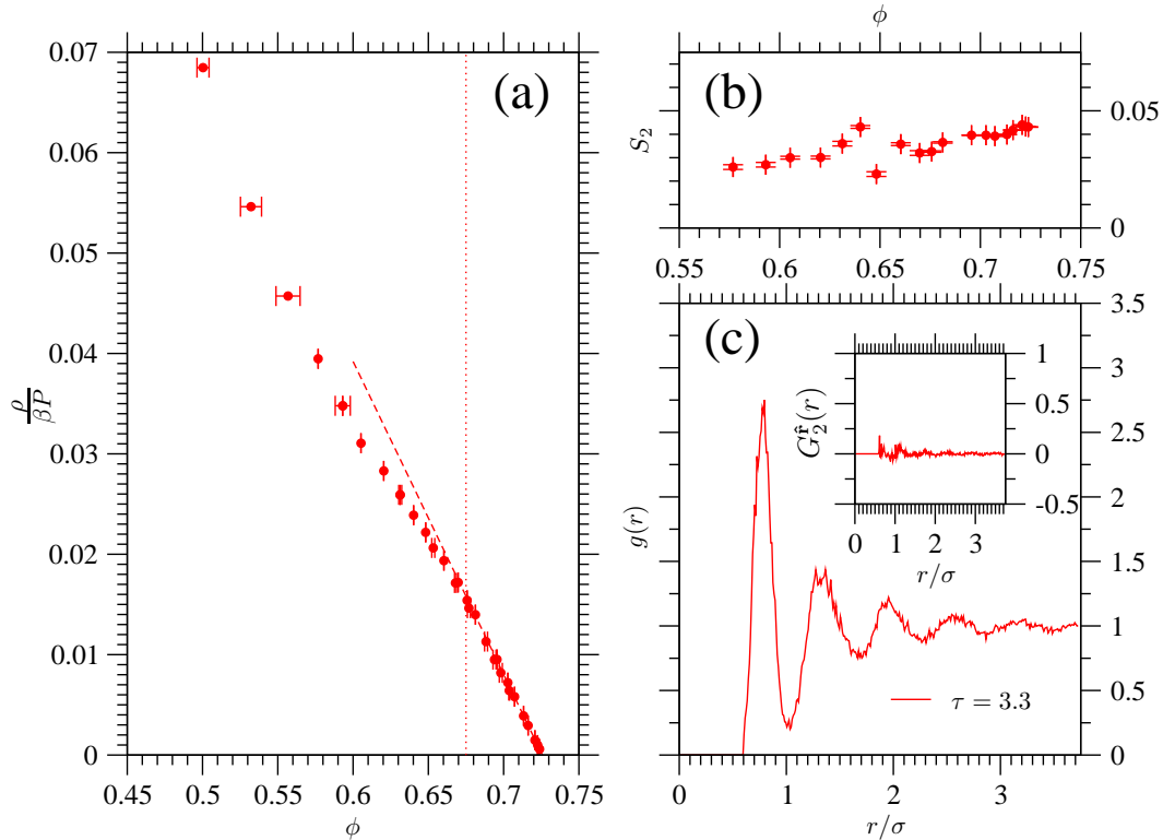
FIG. 14. (a) Inverse compressibility factor \frac{\rho}{\beta P} as a function of volume fraction \phi for lenses with \kappa \simeq 0.63 ; the dotted line indicates the value of \phi beyond which a free-volume-theory-inspired linear fit, the dashed line, was carried out. (b) Nematic order parameter S_2 as a function of volume fraction \phi . (c) Positional pair correlation function g(r) at P^* = 5000 corresponding to \phi = 0.7239 \pm 0.0001 ; the legend gives the corresponding value of \tau ; the inset shows the corresponding bond-orientational pair correlation function G_2^f(r) .
