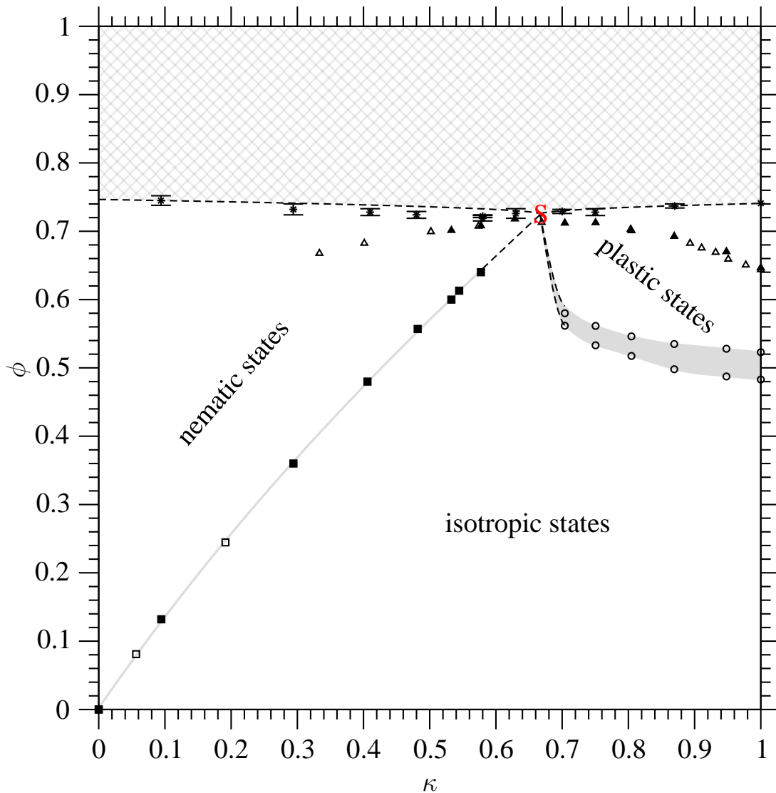
FIG. 16. Crystal-less state diagram for lenses in the plane aspect ratio \kappa — volume fraction \phi . There are three regions where nematic, isotropic and plastic states are (either absolutely or relatively) stablest delimited by: the IN phase transition line(s) and its (their) continuation (empty and filled squares crossed by the gray wide line continued by the black dashed line); the IP phase transition lines and their continuation (empty circles and the gray region within continued by the two black dashed lines); the non-crystalline jammed state volume fraction curve (black asterisks and black dashed line; above, state points within the gray netted region are unachievable). Hypothetically, the latter curve meets with both IN and IP phase transition line continuations at the singular state point marked by a red S. The triangles are data for the MRJ volume fractions of lenses (filled) and hard oblate ellipsoids 20 (empty).
