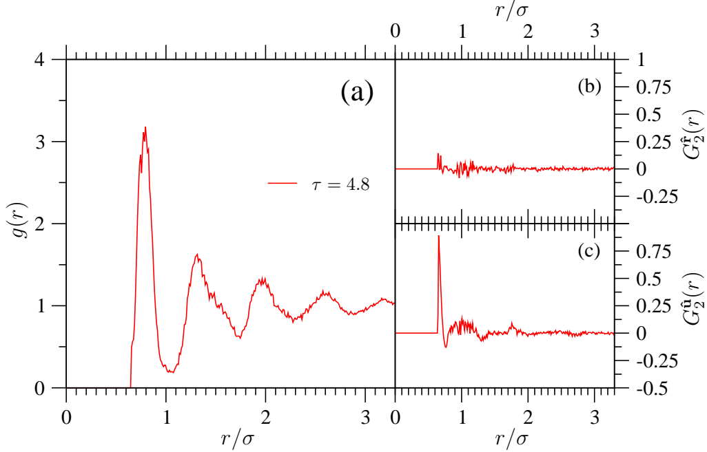
FIG. 13. Pair correlation functions calculated for a system of lenses with \kappa \simeq 0.70 at P^* = 5000 corresponding to \phi = 0.7260 \pm 0.0001 : (a) positional g(r) with the legend giving the corresponding value of \tau ; (b) bond-orientational G_2^f(r) ; (c) orientational G_2^u(r) .
