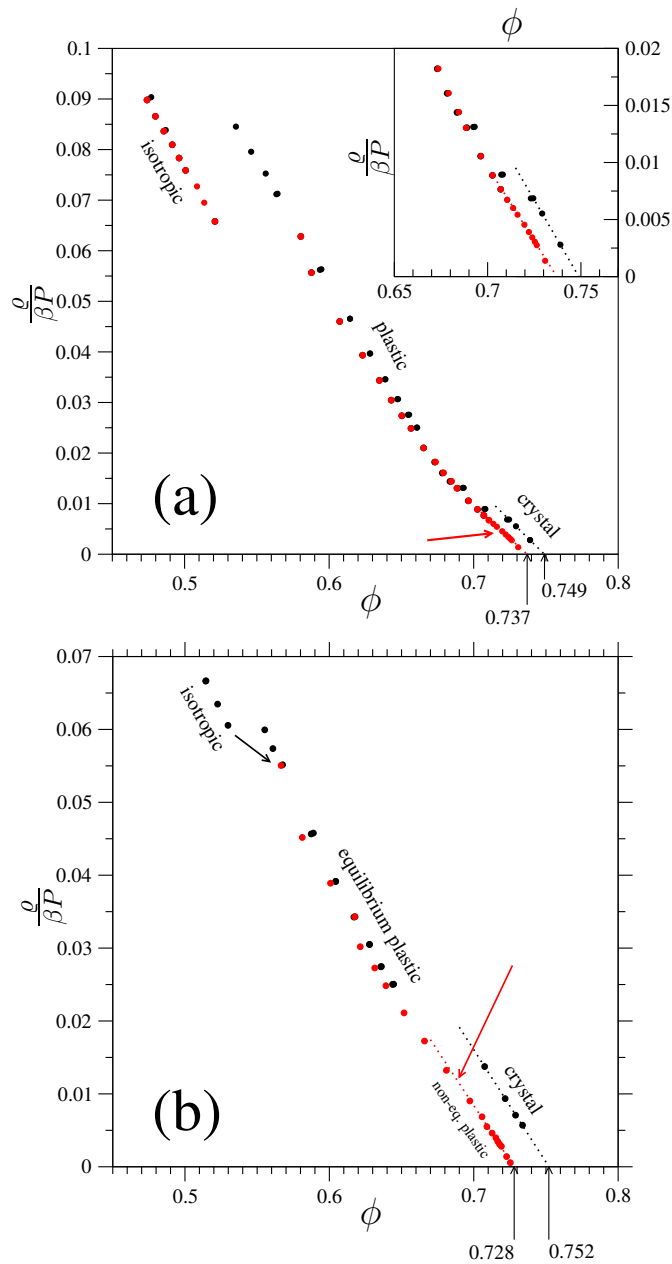
FIG. 8. Inverse compressibility factor \frac{\rho}{\beta P} as a function of volume fraction \phi for lenses with \kappa \simeq 0.87 (a) and for lenses with \kappa \simeq 0.75 (b). Shown are the equilibrium branches obtained by progressive decompression starting from a densest-known orthorhombic configuration (black circles) and the (non-)equilibrium branches obtained by progressive compression starting from a dense isotropic configuration (red or gray circles). The dotted curves are linear, free-volume-theory-inspired, fits over the densest state points. The red (gray) arrow approximately indicates the ‘downturn’ and setting in of this linear behaviour in the compression curve. In (a), the top-right inset zooms in on the high-volume-fraction data. In (b), the black arrow joins that initial isotropic state point with the successive plastic state point.
