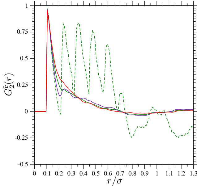
FIG. 5. Bond-orientational pair correlation function G_2^{\mathbf{f}}(r) calculated for a system of lenses with \kappa \simeq 0.094 in a nematic state at P^* = 250 (red or gray full), 350 (green or gray full) and 450 (indigo or dark gray full), and in the C solid phase at P^* = 350 (green or gray dashed).
