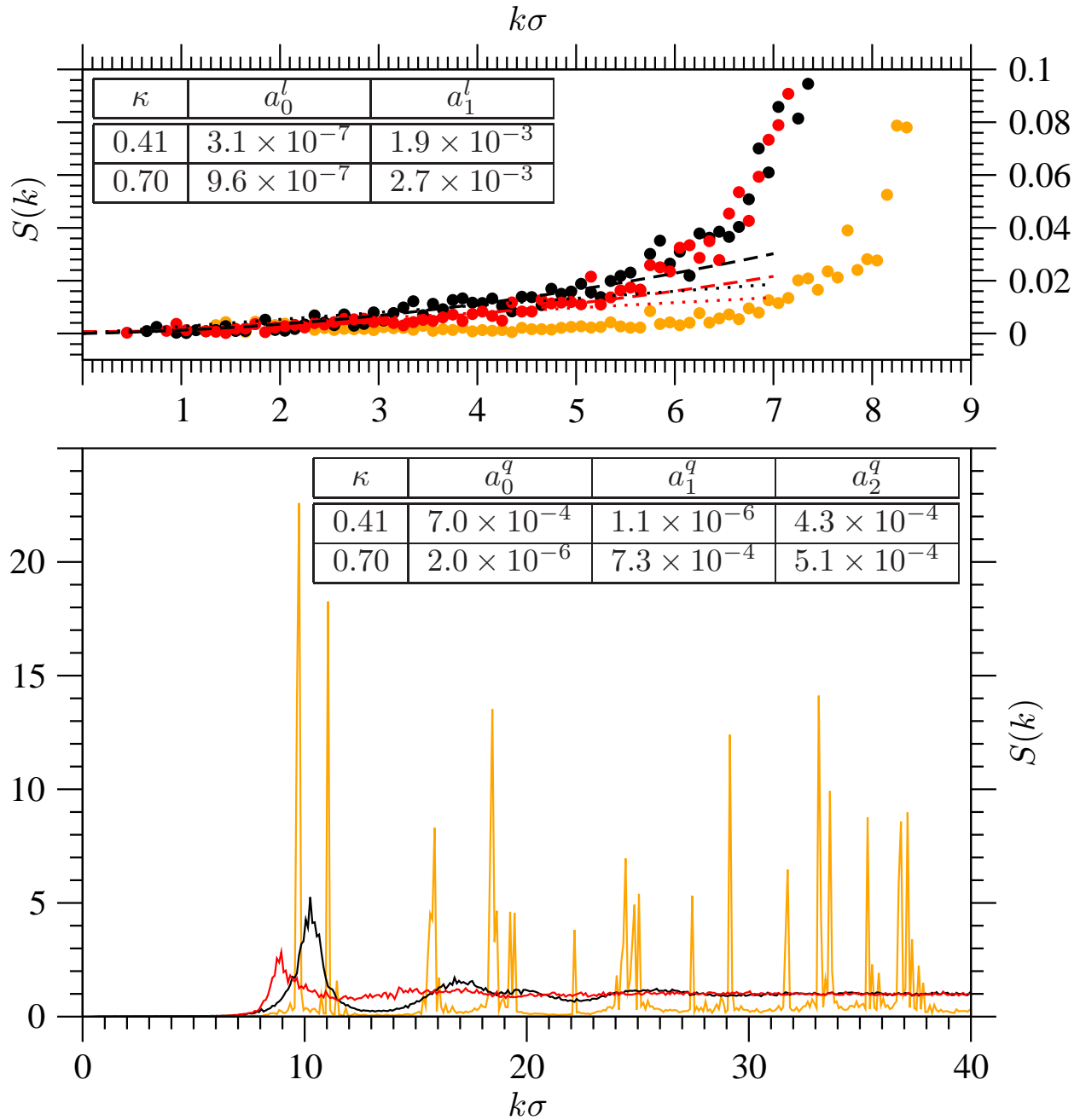
FIG. 15. The structure factor S(k) for three strictly jammed packings of lenses with: \kappa \simeq 0.41 , representative of ‘flat’ lens class with a nematic structure (red or gray line and red or gray circles); \kappa \simeq 0.70 , representative of ‘intermediate’ lens class with an isotropic structure (black curve and black circles); \kappa \simeq 0.87 , representative of ‘globular’ lens class with a plastic structure (orange or light gray curve and orange or light gray circles). The upper panel zooms in on the small- k behaviour while the two inset tables report the coefficients of the linear (dotted curve of the corresponding color) and quadratic (dashed curve of the corresponding color) fits over k\sigma < 5 for the two positionally disordered packings.
