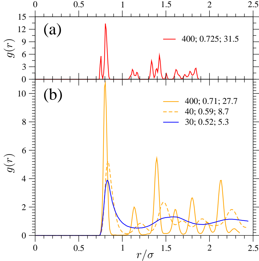
FIG. 9. (a) Positional pair correlation function g(r) for a system of lenses with \kappa \simeq 0.87 in the C solid phase at P^*=400 , \phi=0.725 . (b) Positional pair correlation function g(r) for a system of lenses with \kappa \simeq 0.87 in the P solid phase at P^*=400 , \phi=0.71 (orange or light gray full line) and P^*=40 , \phi=0.59 (orange or light gray dashed line) and in the I fluid phase at P^*=30 , \phi=0.52 (blue or dark gray full line). The third number in each legend gives the corresponding value of \tau .
