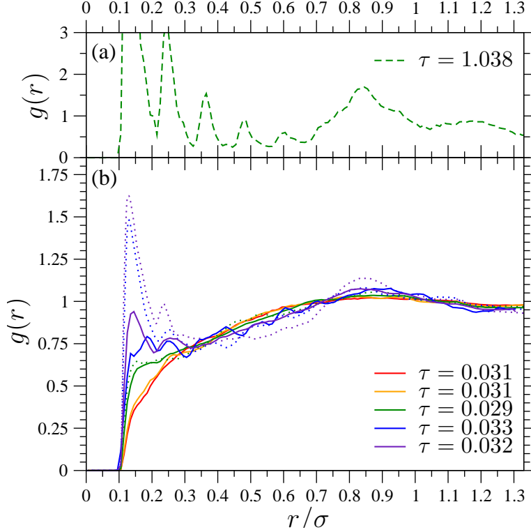
FIG. 4. (a) Positional pair correlation function g(r) calculated for a system of lenses with \kappa \simeq 0.094 in the C solid phase at P^*=350 . The dashed curve refers to a system of N = 432 lenses and was calculated at the end of the corresponding MC run shown in Fig. 3. (b) Positional pair correlation function g(r) calculated for a system of lenses with \kappa \simeq 0.094 in a nematic state at several values of P^* : 250 (red or gray); 300 (orange or light gray); 350 (green or gray dotted and full); 400 (blue or dark gray dotted and full); 450 (indigo or dark gray dotted and full). The dotted curves refer to a system of N = 432 lenses and were calculated at the beginning of the corresponding MC run shown in Fig. 3. The full curves refer to a system of N = 864 lenses and were calculated during a MC run like the one shown in Fig. 3. In (a) and (b) the legends give corresponding values of \tau .
