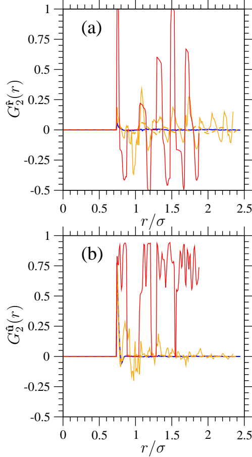
FIG. 10. Bond-orientational pair correlation function G_2^f(r) (a) and orientational pair correlation function G_2^u(r) (b) for a system of lenses with \kappa \simeq 0.87 in the C solid phase at P^*=400 , \phi=0.725 (red or gray wavy full line), in the P solid phase at P^*=400 , \phi=0.71 (orange or light gray full line) and P^*=40 , \phi=0.59 (orange or light gray dashed line) and in the I fluid phase at P^*=30 , \phi=0.52 (blue or dark gray vanishing full line).
