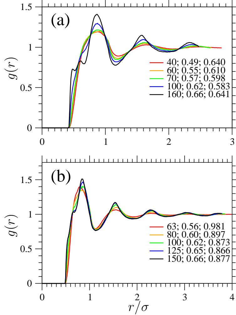
FIG. 7. (a) Positional pair correlation function g(r) calculated for a system of lenses with \kappa \simeq 0.41 at several values of P^* : 40, \phi=0.49 (red or gray); 60, \phi=0.55 (orange or light gray); 70, \phi=0.57 (green or very light gray); 100, \phi=0.62 (blue or dark gray); 160, \phi=0.66 (black). The third number in each legend is the corresponding value of \tau . (b) Positional pair correlation function g(r) calculated for a system of lenses with \kappa \simeq 0.48 at several values of P^* : 63, \phi=0.56 (red or gray); 80, \phi=0.60 (orange or light gray); 100, \phi=0.62 (green or very light gray); 125, \phi=0.65 (blue or dark gray); 150, \phi=0.66 (black). The third number in each legend is the corresponding value of \tau .
