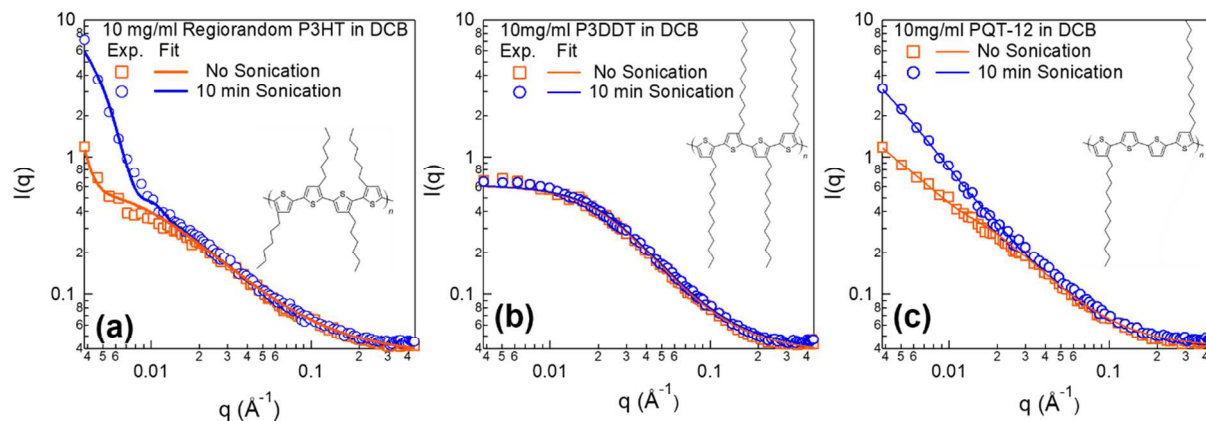
Figure 6. SANS profiles for 10 mg/ml (a) RRa P3HT, (b) P3DDT and (c) PQT-12 in 1,2-dichlorobenzene without and with 10 min sonication. The inset schematics show the molecular structure of each polymer. The models used for fitting the experimental data are the sphere model 51 combined with dissolved polymer with excluded volume for RRa P3HT and also a combined model of parallelepipeds 49,50 with dissolved polymer with excluded volume for PQT-12. The scattering profile of P3DDT is fit with just the dissolved polymer model with excluded volume. 47,48
