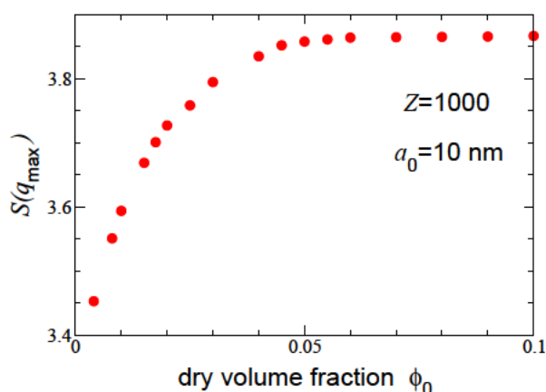
Fig. 9 Main peak height of static structure factor S(q_{max}) vs. dry volume fraction \phi_0 for same systems as represented in Figs. 7 and 8. With increasing concentration, pair correlations strengthen until, near particle overlap ( \phi_0 \approx 0.06 ), the structure saturates.
