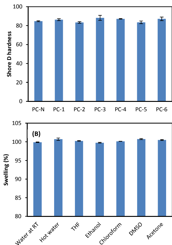
Fig. 7. (A) Shore D hardness of BPA-free PCs prepared from DTMPC (0.33 mmol) by various catalytic conditions at 130°C. PC-N was purchased from Nalgen as a PC control. PC-1; 1.7 \mu mol DBU and 3.5 \mu mol 1,3PDO, PC-2; 1.7 \mu mol DBU and 35 \mu mol 1,3PDO, PC-3; 1.7 \mu mol DBU and 35 \mu mol 1,2PDO, PC-4; 1.7 \mu mol DBU and 24 \mu mol 1,6HDO, PC-5; 0.09 \mu mol TBD and 14 \mu mol 1,3PDO, and PC-6; 0.18 \mu mol TBD and 28 \mu mol 1,3PDO. (B) Swelling properties of BPA-free PCs prepared by using various solvents and conditions. BPA-free PC was prepared from DTMPC (0.33 mmol) by 1.7 \mu mol DBU and 35 \mu mol 1,3PDO at 130°C. The swelling was compared from 100% as the original size.
