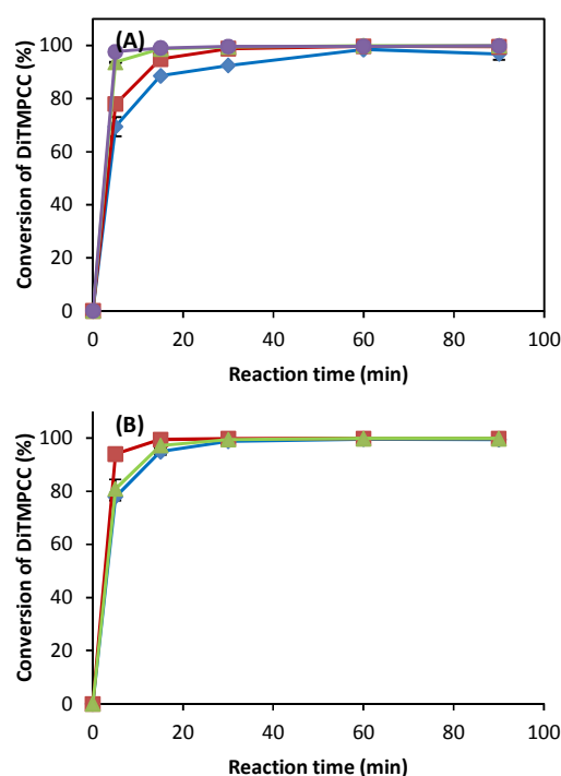
Fig. 2. Synthesis of BPA-free PC from DTMPCC (100 mg, 0.33 mmol) by ROP under various conditions. A) Effect of amount of chain transfer (1,3-PDO) using 1.7 \mu\text{mol} DBU with 3.5 \mu\text{mol} ( \blacklozenge ), 35 \mu\text{mol} ( \blacksquare ), 70 \mu\text{mol} ( \blacktriangle ), and 140 \mu\text{mol} ( \bullet ) of 1,3PDO at 130°C. (B) Effect of chain transfers using 1.7 \mu\text{mol} DBU with 35 \mu\text{mol} 1,3PDO ( \blacklozenge ), 35 \mu\text{mol} 1,2PDO ( \blacksquare ) and 35 \mu\text{mol} 1,6HDO ( \blacktriangle ) at 130°C.
