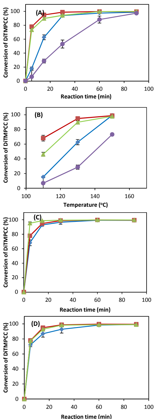
Fig. 1. Synthesis of BPA-free PC from DTMPCC (100 mg, 0.33 mmol) by ROP under various conditions. Effect of (A) catalyst system at 130°C and (B) temperature at 15 min in presence of 8.2 \mu\text{mol} DMAP and 35 \mu\text{mol} 1,3PDO ( \blacklozenge ), 1.7 \mu\text{mol} DBU and 35 \mu\text{mol} 1,3PDO ( \blacksquare ), 0.09 \mu\text{mol} TBD and 35 \mu\text{mol} 1,3PDO ( \blacktriangle ), and 7.2 \mu\text{mol} TEA and 35 \mu\text{mol} 1,3PDO ( \bullet ). C) Effect of temperature under condition of 1.7 \mu\text{mol} DBU and 35 \mu\text{mol} 1,3-PDO at 110°C ( \blacklozenge ), 130°C ( \blacksquare ) and 150°C ( \blacktriangle ). D) Effect of catalyst amount with 0.67 \mu\text{mol} DBU and 35 \mu\text{mol} 1,3PDO ( \blacklozenge ), 1.2 \mu\text{mol} DBU and 35 \mu\text{mol} 1,3PDO, ( \blacktriangle ) 1.7 \mu\text{mol} DBU and 35 \mu\text{mol} 1,3PDO ( \blacksquare ) at 130°C.
