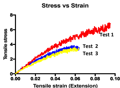
Fig. 6. Tensile mechanical properties of BPA-free PC (PC-T) prepared from 0.33 mmol DTMPC, 0.09 \mu\text{mol} TBD and 14 \mu\text{mol} 1,3-PDO at 130°C for 1 hr.
