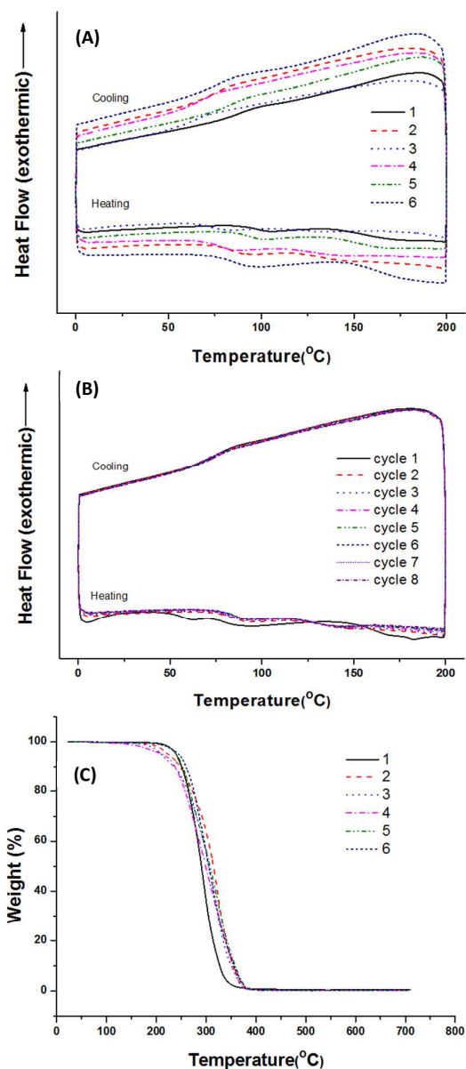
Fig. 5. Thermal properties of the BPA-free PCs prepared from DTMPC (0.33 mmol) by different conditions. (A) DSC graphs for BPA-free PC samples prepared using (1) 1.7 \mu\text{mol} DBU and 3.5 \mu\text{mol} 1,3PDO, (2) 1.7 \mu\text{mol} DBU and 35 \mu\text{mol} 1,3PDO, (3) 1.7 \mu\text{mol} DBU and 70 \mu\text{mol} 1,3PDO, (4) 1.7 \mu\text{mol} DBU and 35 \mu\text{mol} 1,2PDO, (5) 1.7 \mu\text{mol} DBU and 24 \mu\text{mol} 1,6HDO, (6) 1.7 \mu\text{mol} DBU and 140 \mu\text{mol} 1,3PDO at 130°C. (B) DSC cycling graph of BPA-free PC prepared by 1.7 \mu\text{mol} DBU and 35 \mu\text{mol} 1,3-PDO at 130°C. (C) TGA graphs for PC samples prepared by the same condition with (A) DSC samples.
