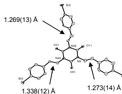
Figure 1. ORTEP representation of 4-Br at the 50 % probability level with selected bond lengths indicated. Hydrogen atoms have been omitted for clarity.
