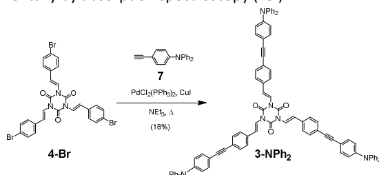
Scheme 3. Synthesis of 3-NPh 2 .
