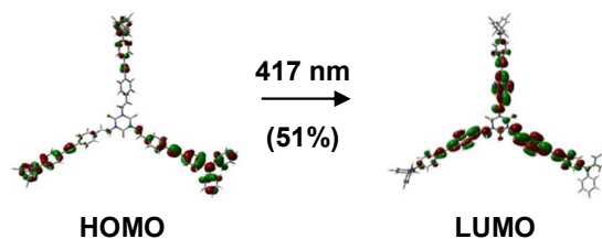
Figure 3. Plots of the frontier molecular orbitals for 3-NPh 2 primarily involved in the main excitation underlying the first allowed transition. Contour values are \pm 0.03 ( \text{e}/\text{bohr}^3 ) 1/2 .
