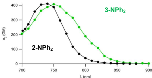
Figure 4. Two-photon absorption spectra of 2-NPh 2 and 3-NPh 2 in dichloromethane (20 °C) in the near-IR range.
