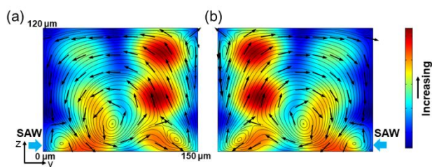
Figure 2. Simulated acoustic streaming patterns and the distribution of acoustic pressure in the microchannel when the SAW is from either of the IDTs. Red and blue colors indicate high and low magnitudes of acoustic pressure, respectively. The direction of acoustic streaming lines is indicated by the black arrows. (a) The SAW coming from the left side generates a large, counterclockwise vortex in the middle of the channel and some smaller vortices near the edges, whereas (b) the SAW coming from the right side generates a clockwise vortex in the middle of the channel and also some smaller vortices. Moreover, the SAW coming from either side forms a pressure node near the middle of the channel.
