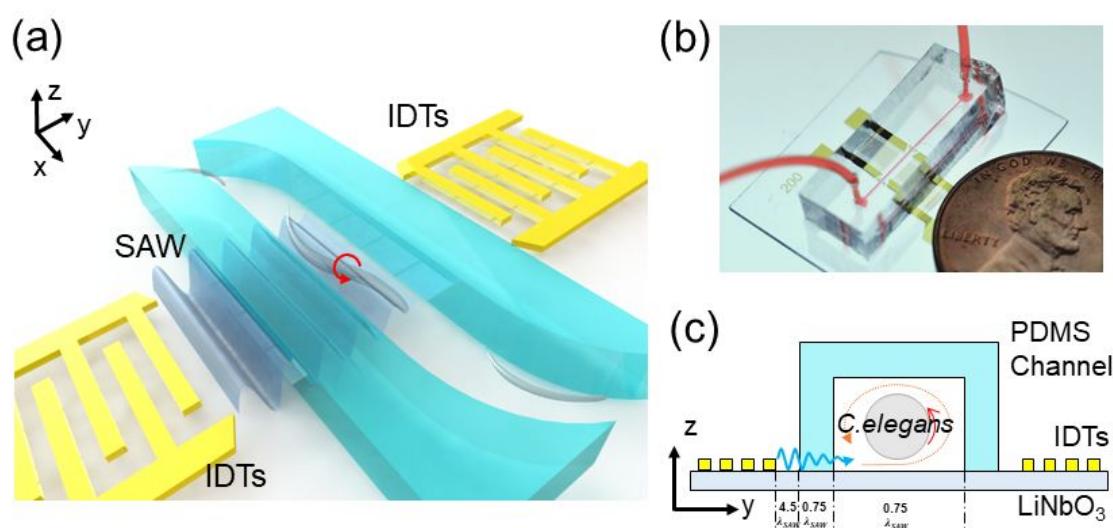
Figure 1. Design and working concept of the SAW-based C. elegans rotation device. (a) Schematic and (b) Photograph of the device. (c) Working principle of the SAW-based rotation device in y - z side view. Here the \lambda_{SAW} is 200\ \mu\text{m} . The SAW generated from the activated left IDT travels into the microchannel and induces acoustic streaming, which can rotate C. elegans along the streaming direction.
