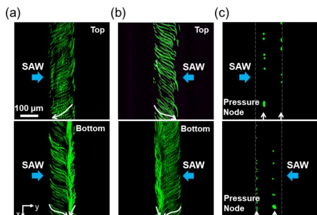
Figure 3. Fluorescent images showing the acoustic streaming pattern and the distribution of acoustic pressure in the microchannel, when the IDT on one side is activated. Green fluorescence tracing of 1 \mu\text{m} particles in top and bottom planes of the microchannel when SAW came from (a) the left IDT and (b) the right IDT, which displays the streaming inside the microchannel. White arrows show the moving direction of particles. (c) Green fluorescence distribution of 10 \mu\text{m} particles when SAW came from the left or right IDTs, which shows the positions of pressure node inside the microchannel, as pointed by white arrows.
