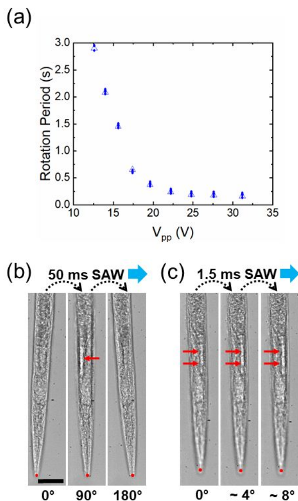
Figure 5. (a) Plot of the rotation period of one C. elegans versus the driving voltage applied to the left IDT. The plot suggests that we can rotate C. elegans in a large speed range with our SAW device. Image sequences showing the stepwise rotation of C. elegans when the IDT was supplied with pulsed signals of (b) 50 ms duration and (c) 1.5 ms duration. Red dots label the position of worm's tip to show there is no drifting. Red arrows point out the differences among figures, which result from rotation. Scale bar: 50 \mu\text{m} .
