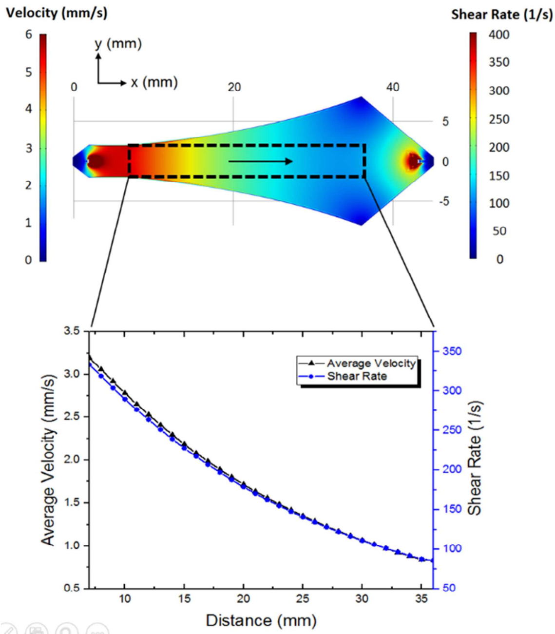
Figure 2. Flow velocity and shear rate contours on a 2D plane 5 \mu\text{m} above the bottom surface. Shown is the region of interest (ROI, dashed line) in which the data analyses were performed. As shown graphically, there is a 3-fold reduction in average velocity and shear rate through the defined ROI. Arrow indicates flow direction.
