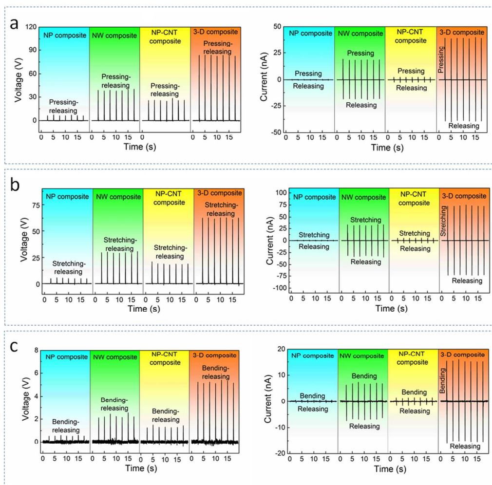
Fig. 4 Piezoelectric responses of the NP, NW, NP-CNT and 3-D composites with multiple deformation modes. (a) The output voltages and currents of different composites under compressing-releasing mode with 8% strain. (b) The output voltages and currents of the composites under stretching-releasing mode with 15% strain. (c) The output voltages and currents of the samples under bending by a displacement of 2 cm from an original length of 5 cm. Overall, the 3-D composites exhibit superior performance compared to the other composites with low-dimensional fillers.
