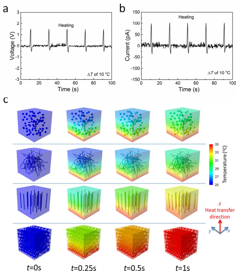
Fig. 5 Pyroelectric responses of the composites. (a,b) The pyroelectric output voltage and current of the 3-D composites under a temperature fluctuation of 10 °C. (c) Finite element modeling of the heat transfer in the composites with different ceramic fillers. A hot plate as a heat source of a temperature 35 °C, 10 °C higher than the ambient temperature, is placed at the bottom of the composites. Heat transfers along the z direction from the bottom to the top of the samples. For each type of ceramic fillers, four different snapshots in the heat transfer process are displayed. The 3-D interconnected PZT ceramic-based composite exhibits significantly faster heat transfer than other composites.
