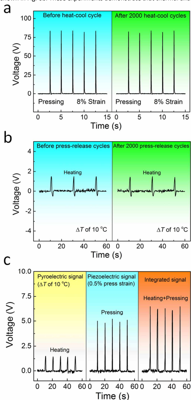
Fig. 6 Pyroelectric, piezoelectric and concurrent piezo-/pyro-electric responses of the 3-D composites. (a,b) The piezoelectric and pyroelectric voltages of the 3-D composites before and after 2000 heating-cooling cycles ( \Delta T of 10 °C) and 2000 pressing-releasing cycles (8% strain), respectively. (c) The individual and integrated piezoelectric-pyroelectric output voltages of the 3-D composites, showing the superimposable piezo/pyroelectric effect.
