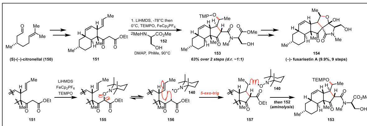
Scheme 17. Theodorakis' use of TEMPO for the synthesis (-)- fusarisetin A (154)
