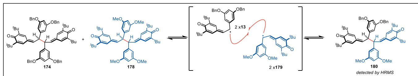
Scheme 21. Thermal crossover experiment suggests persistent radical equilibrium.
