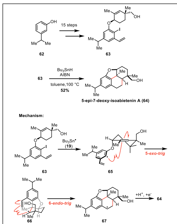
Scheme 9. Zhang's total synthesis of 5-epi-7-deoxy-isoabietaen A ( 64 ).
