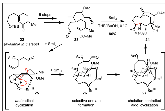
Scheme 3. Procter's approach to pleuromutilin analogues.
