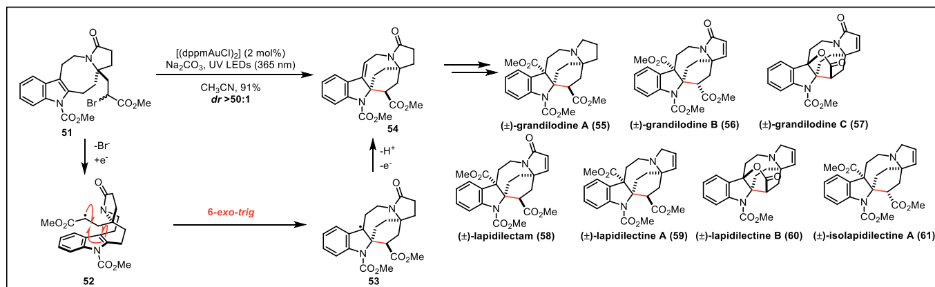
Scheme 8. Echavarren's unified approach to pyrroloazocine indole alkaloids using photoredox catalysis.
