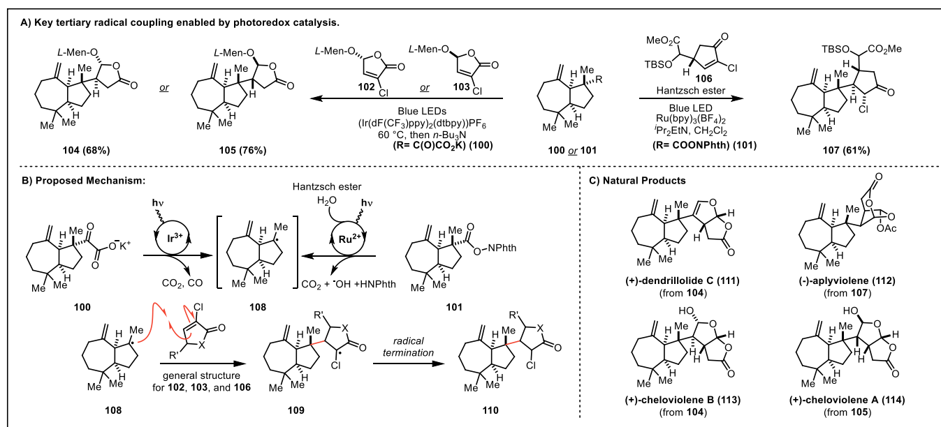
Scheme 13. Overman's tertiary radical coupling to set vicinal stereocenters and access marine sponge terpenoids.
