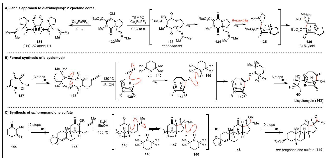
Scheme 16. Jahn’s use of TEMPO to establish persistent radical equilibria for the synthesis of natural products. R = TEMPO
