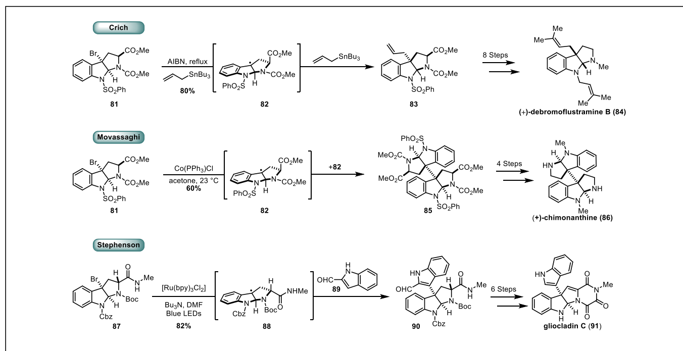
Scheme 11. Approaches to pyrroloindolinyl radicals starting from bromopyrroloindoline precursors.
