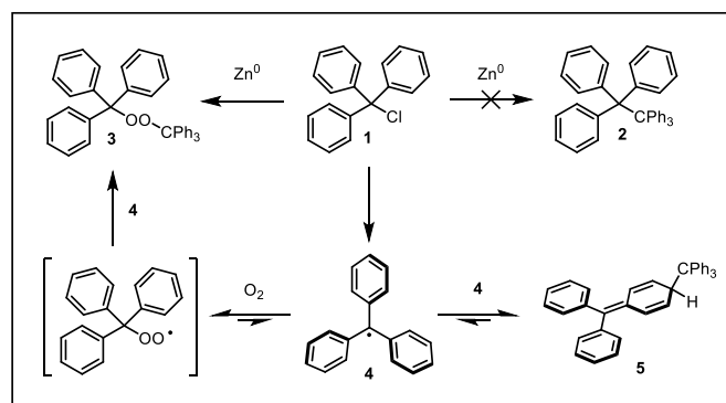
Scheme 1. Gomberg's discovery of the triphenylmethyl radical.
