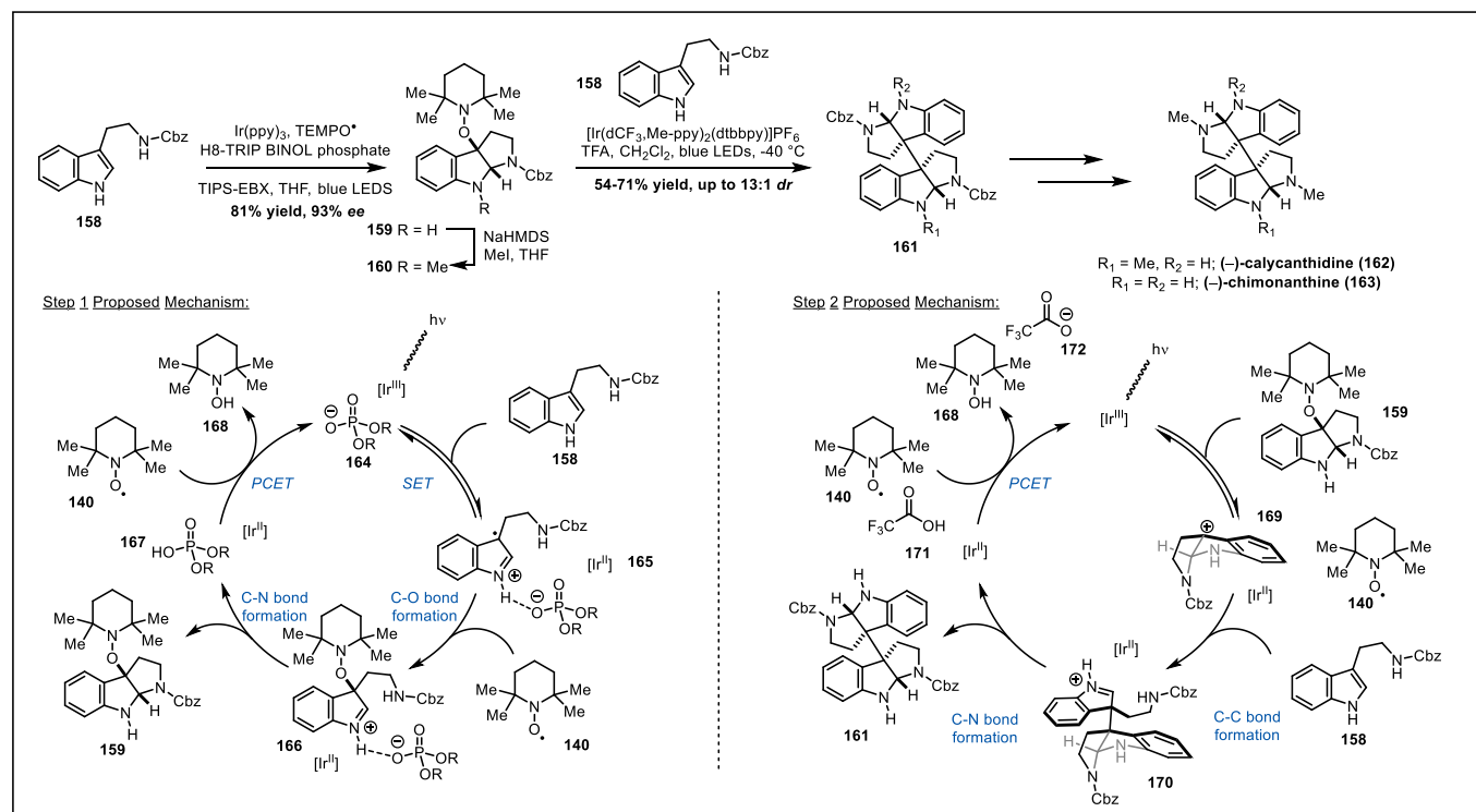
Scheme 18. Knowles' use of TEMPO for the synthesis of pyrroloindoline natural products.
