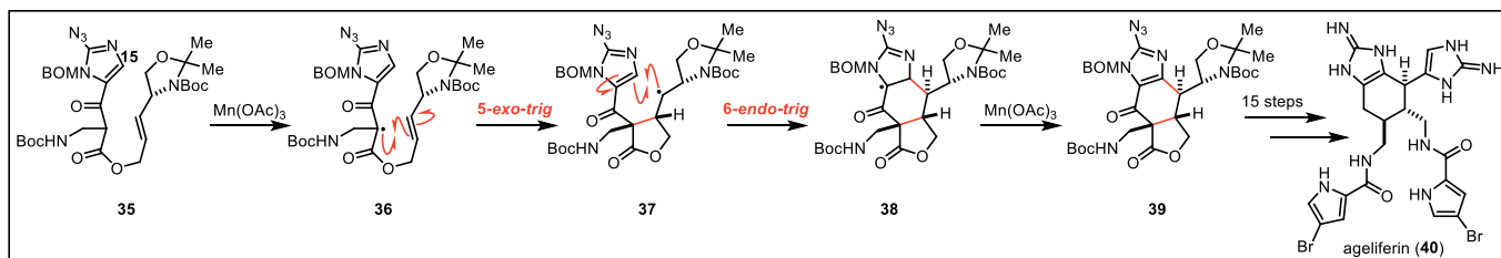
Scheme 5. Chen's asymmetric synthesis of ageliferin ( 40 ) utilizing a tandem 5-exo/6-endo cyclization strategy.
