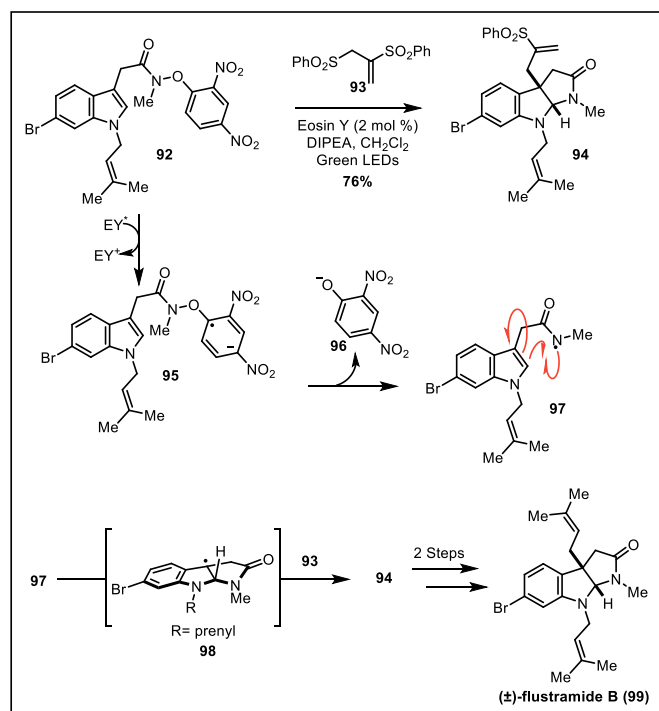
Scheme 12. Wang's synthesis of (±)-flustramide B ( 99 ).
