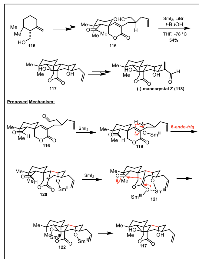
Scheme 14. Reisman's synthesis of maeocrystal Z ( 118 ).
