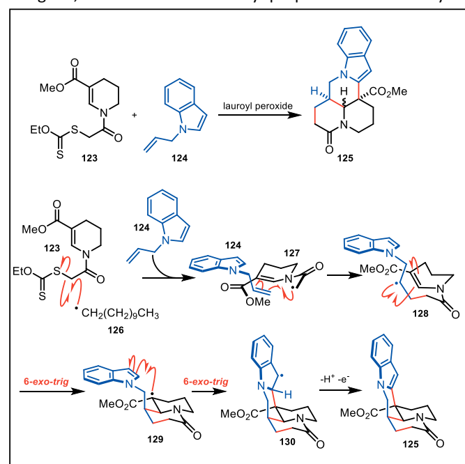
Scheme 15. Miranda’s synthesis of matrine analogues.
