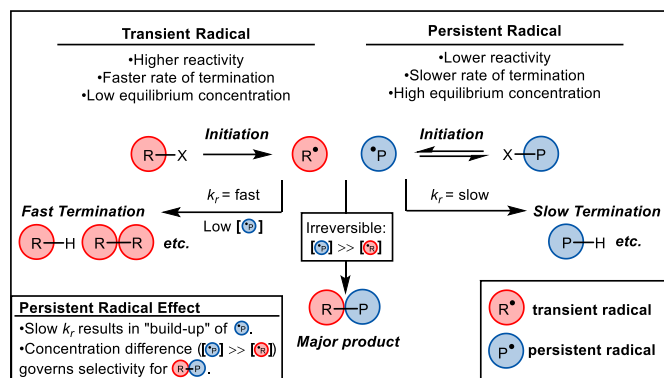
Figure 2. Generic depiction of the persistent radical effect.
