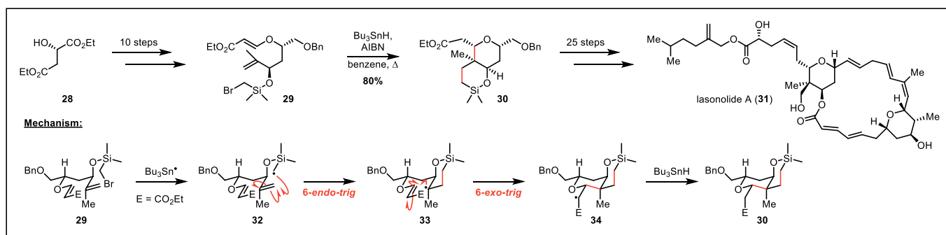
Scheme 4. Song's approach to lasonolide A ( 31 ) featuring a 6-endo/6-exo tandem cyclization.
