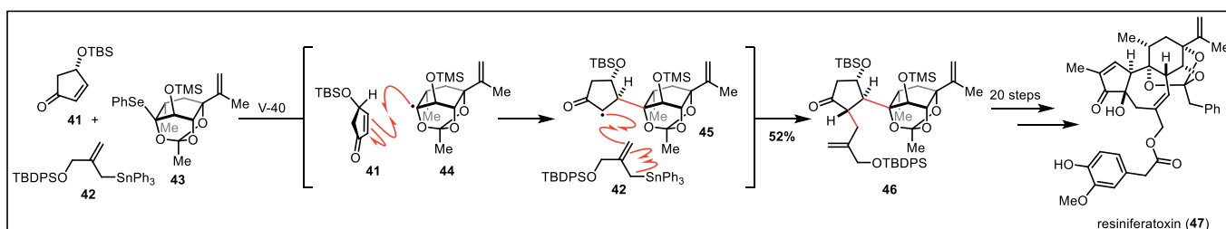
Scheme 6. Inoue's synthesis of resiniferatoxin ( 47 ) featuring a 3-component radical coupling strategy.
