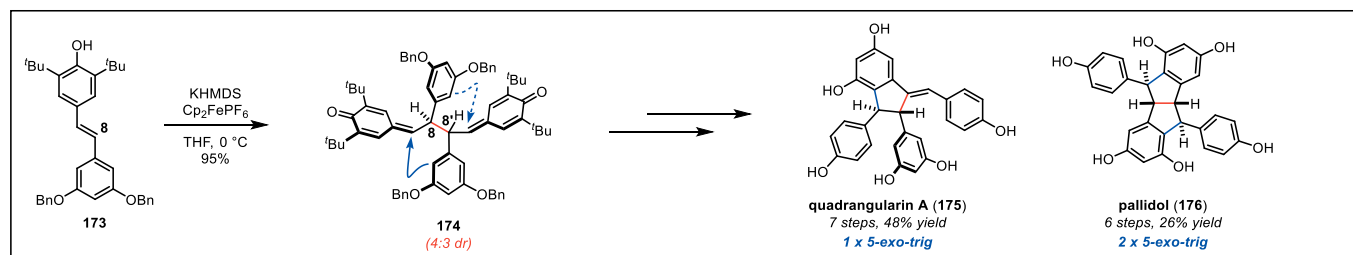
Scheme 19. Stephenson's biomimetic synthesis of quadrangularin A ( 175 ) and pallidol ( 176 ).
