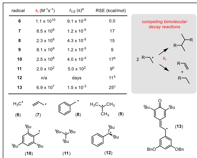
Figure 1. Selected kinetic and thermodynamic parameters of some C-centered radicals. a Lifetimes are based upon a radical concentration of 10^{-5} M. b Calculated using CBS-QB3. 9 c This RSE is derived from the BDE of the phenolic tautomer that gives rise to 13 .
