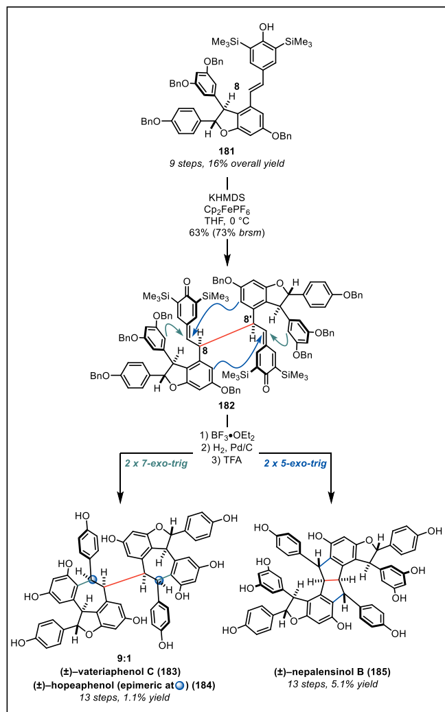
Scheme 22. Synthesis of resveratrol tetramers via a persistent radical equilibrium.
