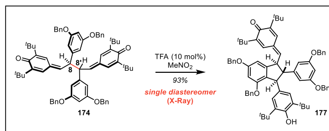
Scheme 20. Diastereoconvergent cyclization with substoichiometric Bronsted acid.
