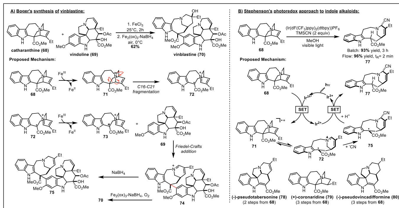
Scheme 10. Approaches leveraging the fragmentation of catharanthine ( 68 ) to access indole alkaloid natural products.
