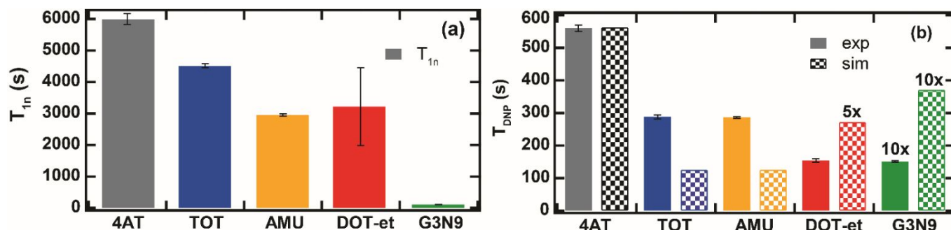
Figure 3. Experimentally determined T_{1n} (a) and T_{DNP} (b-solid) for each radical. (b) A comparison of experimental (solid) and simulated (checkered) T_{DNP} for each case. The values for G3N9 in (b) are 10x to ease visualization, while those of the simulated DOT-et T_{DNP} are magnified 5x. Here the simulated T_{DNP} is extracted from the mono-exponential fit of the total nuclear spin polarization shown in figure S10, where K_{sd} = 0.001 Hz, \Delta B = 1 kHz, and the values of t_{een} are extracted from equation 7 for each radical. Further details of how t_{een} and T_{DNP} were calculated can be found in the ESI.
