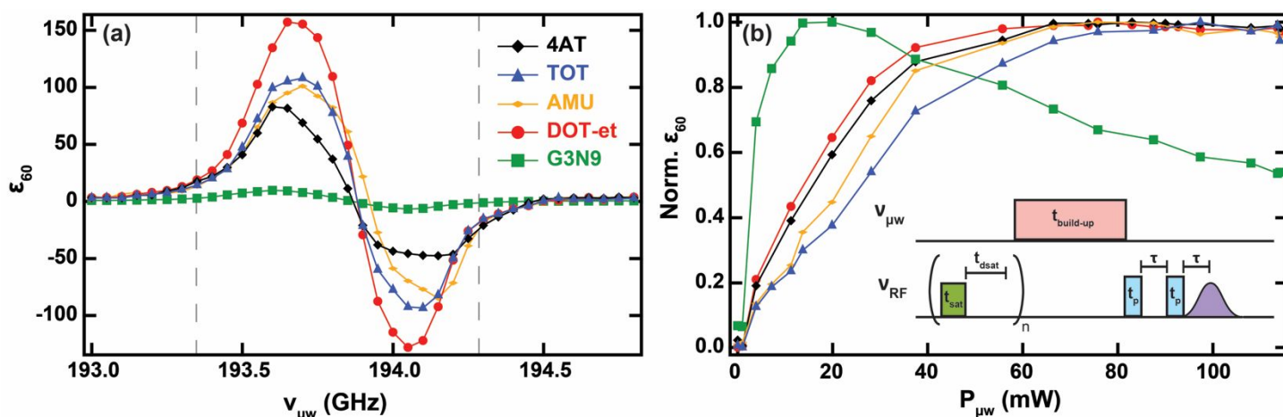
Figure 2. (a) DNP profiles at 4K and at 7 T for 10 mM 4AT (black diamond), 5 mM TOT (blue triangle), 5 mM AMU (yellow small diamond), 3.33 mM DOT-et (red circle), and 1.11 mM G3N9 (green square) in 6:3:1 d_8 -glycerol: D_2O : H_2O . The dashed lines represent the width of the allowed EPR spectrum. (b) The normalized DNP power curves acquired with \mu\text{w} irradiation at 193.65 GHz. All data was acquired with a saturation recovery solid echo pulse sequence as shown in the inset of (b) with t_p = 2.5 \mu\text{s} , \tau = 110 \mu\text{s} , t_{\text{sat}} = 2.4 \mu\text{s} , t_{\text{dsat}} = 380 \mu\text{s} , n = 10 , and t_{\text{build-up}} = 60 \text{ s} .
