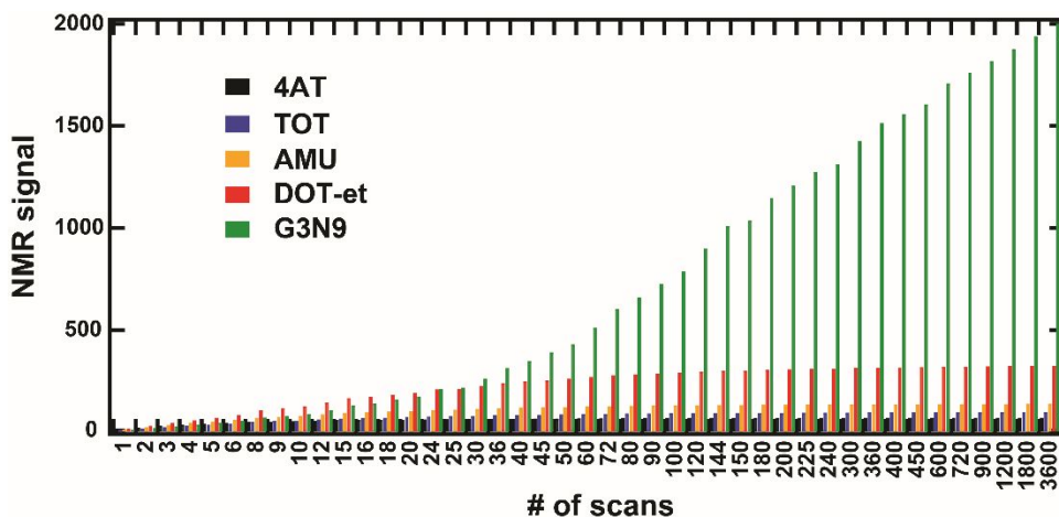
Figure 6. Simulated NMR signal ( M_{z,on}(t) ) after signal averaging for a total timeframe of 3600 sec, where the t_{build-up} * \text{number of scans} = \text{total timeframe} . Equation 2 was used and for this simulation with each radical's respective \epsilon_{eq} and T_{DNP} , where M_{z,on}(t) * \text{number of scans} produced the reported NMR signal.
