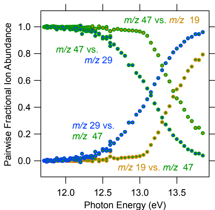
Figure 2. Pairwise fractional ion abundances for the m/z = 29 vs. 47 and m/z = 19 vs. 47 ions. The gradual rise exhibited by the first pair suggests parallel formation of these species, while the m/z = 19 ion is likely formed in a consecutive dissociation step from the m/z = 47 ion – apart from a small fraction that very gradually increases to a few percent in the 12–13 eV energy range.
