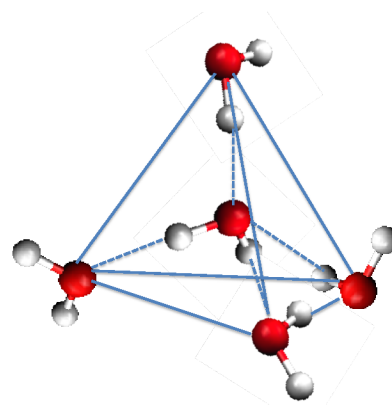
Fig. 1 Tetrahedral water configuration
