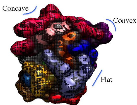
Fig. 2 Illustration of different surface curvature regions of CALB: concave (1 on surface curvature scale), flat (3 on scale), and convex (5 on scale).
