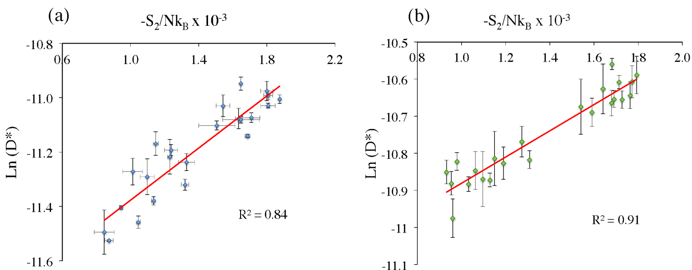
Fig. 10 Logarithmic relationship between hydration shell water diffusivity and pair entropy, as described in the Rosenfeld relationship (Eq. 9), in the presence of (a) SPC/E water model and (b) TIP4P water model.
